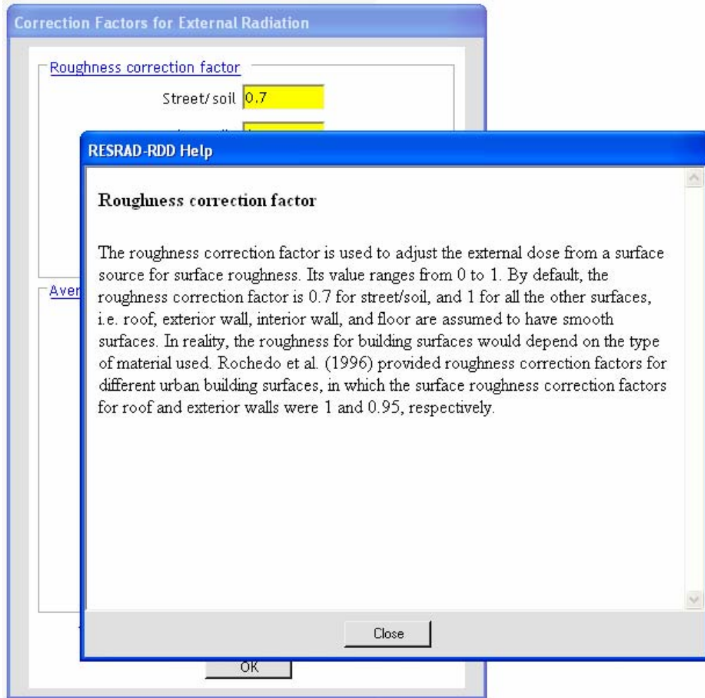
FIGURE 12.10 Additional Explanation for Roughness Correction Factor
