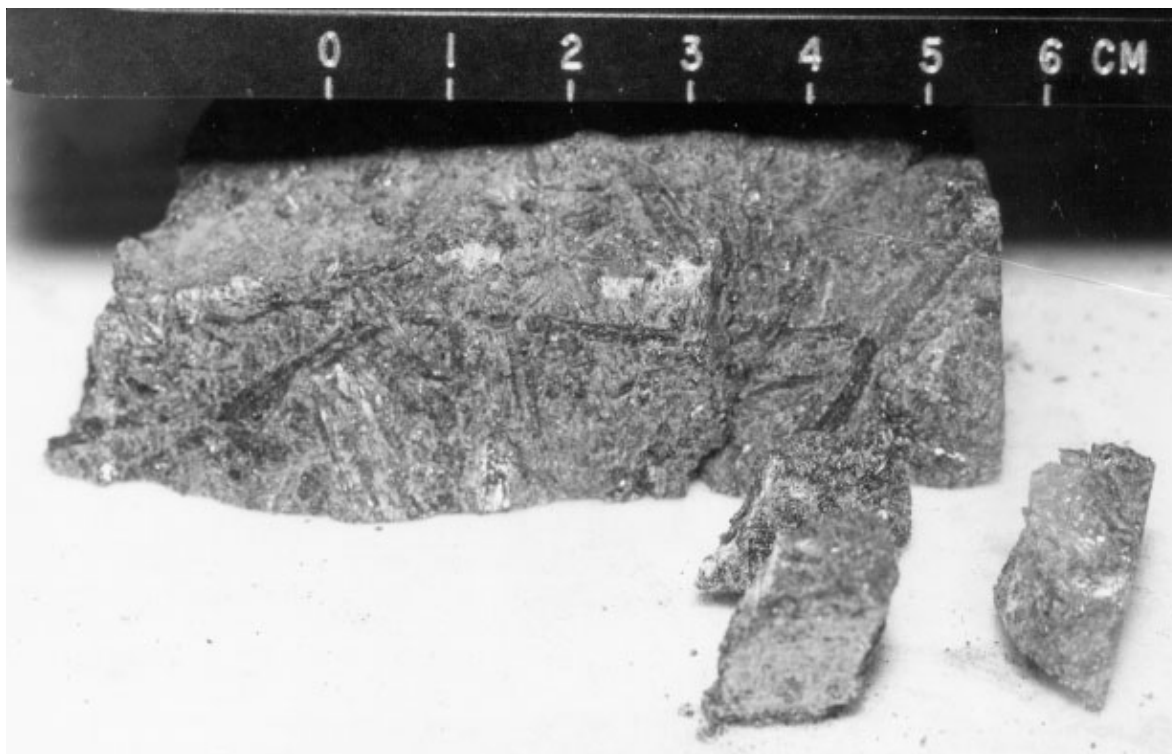
Figure 1: Photo of 12021,36 showing elongate pyroxene in broken surface.
