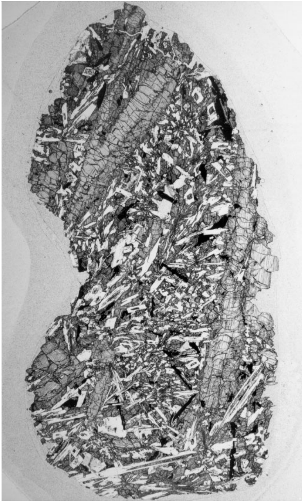
Figure 2: Photomicrograph of thin section of 12021,3 showing elongate and sector-zoned pyroxene. Field of view is 3 cm. NASA # S70-25401.
