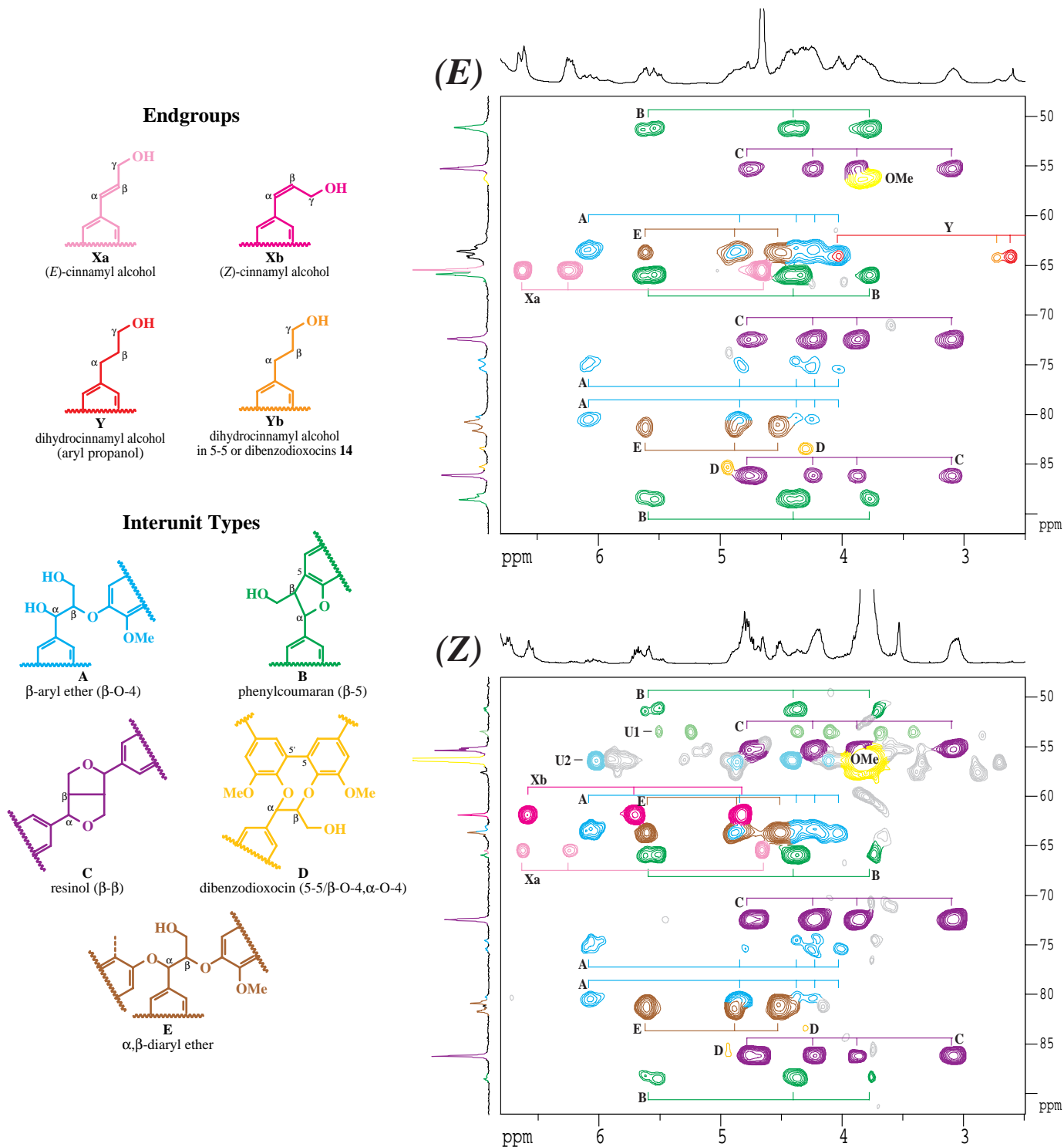
Figure 1. Sidechain region of 2D HMQC-TOCSY 29 spectra of synthetic lignins prepared from ( E )- and ( Z )-coniferyl alcohols. Such spectra correlate a carbon with its attached proton and all protons within the same coupling network as that attached proton. They consequently give redundant information which is particularly valuable in tracing out lignin substructures. Lignin units A-E are identified, along with coniferyl alcohol endgroups Xa , the ( E )-cinnamyl alcohol sidechain, and Xb , this ( Z )-sidechain. Contours at carbon frequencies labeled U1 and U2 are currently unassigned. The small amount of dihydroconiferyl alcohol endgroups Y in the ( E )-coniferyl alcohol lignin are from a 2% dihydroconiferyl alcohol impurity in the monomer. The ( E )-cinnamyl alcohol endgroups Xa (~5% of the Xb contours) in the ( Z )-coniferyl alcohol polymer are from the 2% ( E )-coniferyl alcohol that was in that monomer. A clearer color version of this figure is available from:
