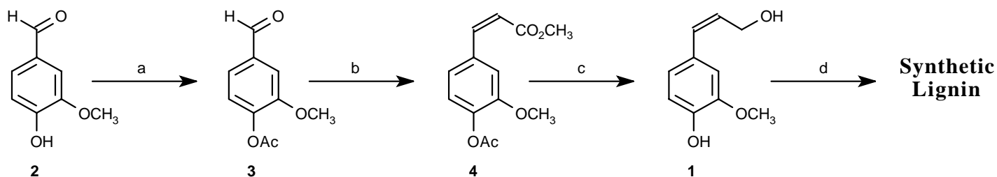
Scheme 1. Synthetic scheme for ( Z )-coniferyl alcohol 1 . Reagents and conditions: a: Acetic anhydride, pyridine, r.t.; b: bis(2,2,2-trifluoroethyl) (methoxycarbonylmethyl)phosphonate, 18-crown-6, KN(TMS)_2 , THF, -78 °C; c: DIBAL, toluene, 0 °C; d: peroxidase, H_2O_2 .
