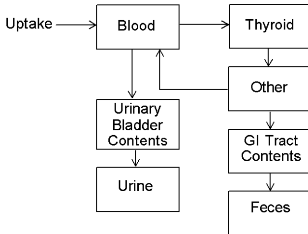
Figure 5.1. Structure of the model for iodine used in ICRP Publication 30 (1979) and current ICRP documents.
