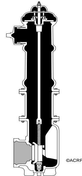
Slide Gate Hydrant
