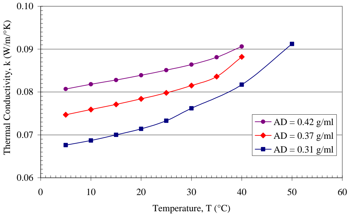
Thermal Conductivity of Westvaco Activated Carbon Product
