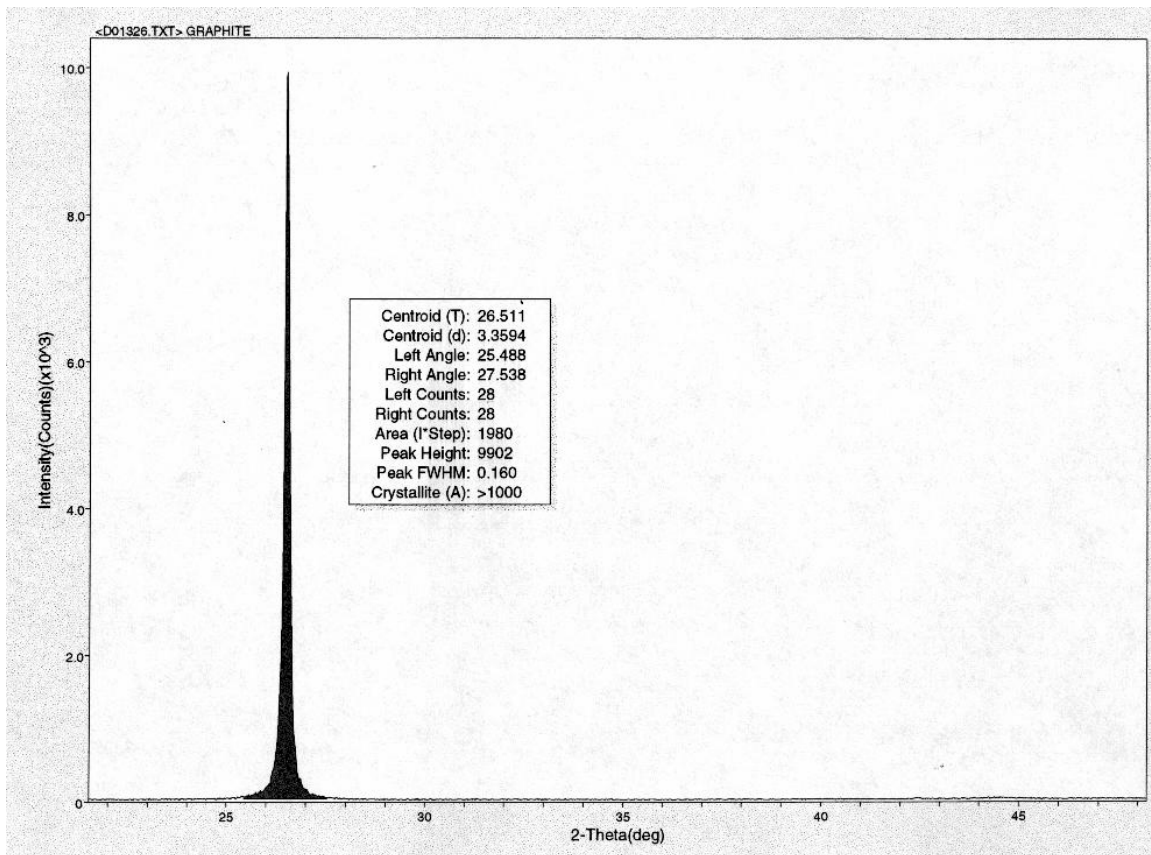
Figure 9. X-ray diffraction pattern from 2\theta = 21^\circ to 2\theta = 48^\circ showing the (002) peak for artificial graphite
