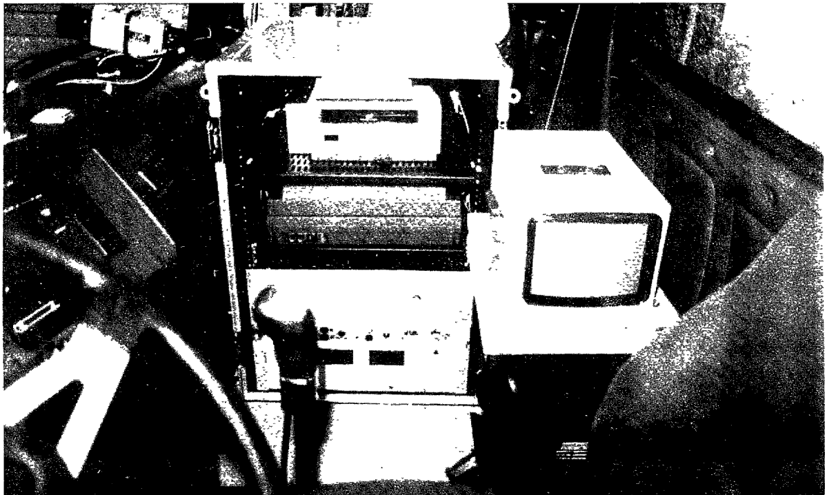
Figure 5. Instrumentation in cab
