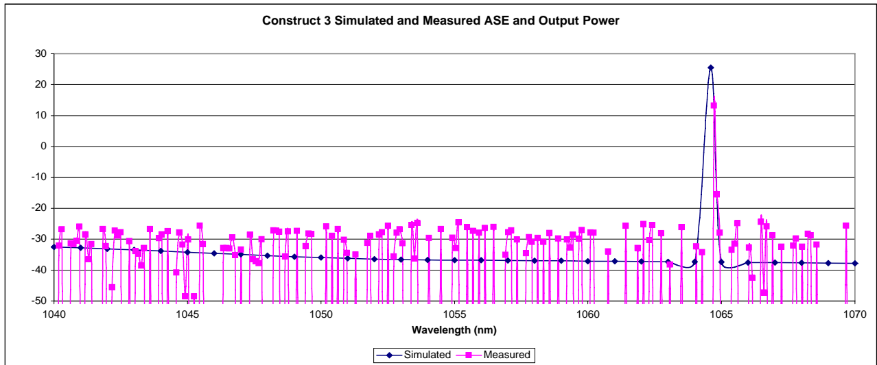
Figure 10. Comparison of simulated performance to experimental results of Yb doped fiber amplifier.
