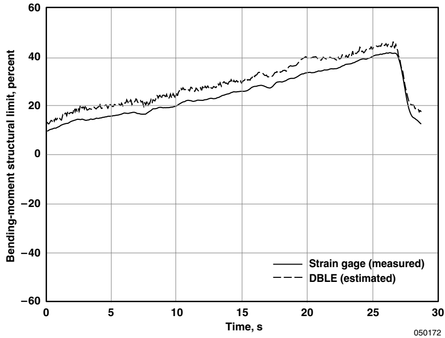
(b) Wing-fold bending moment.
