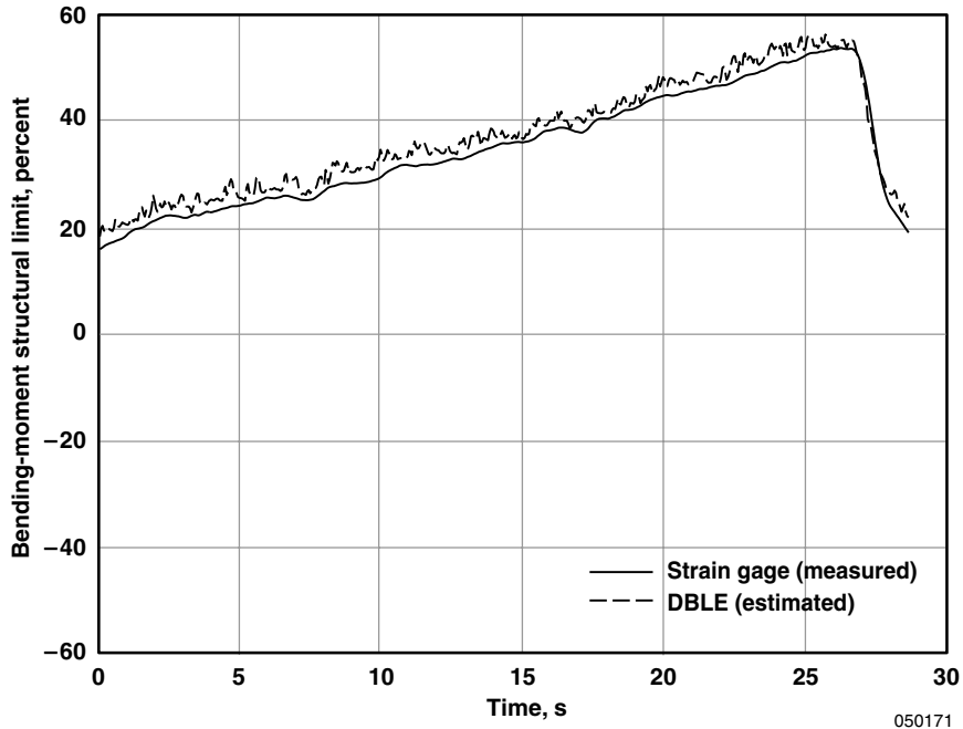
(a) Wing-root bending moment.
