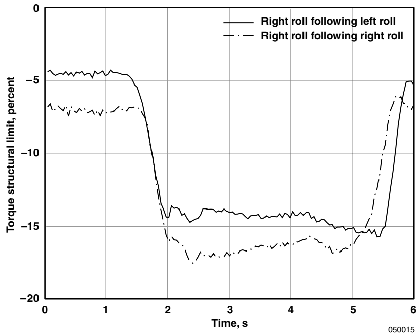
(c) Wing-root torque.
