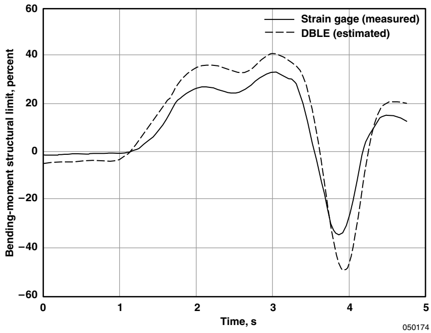
(b) Wing-fold bending moment.
