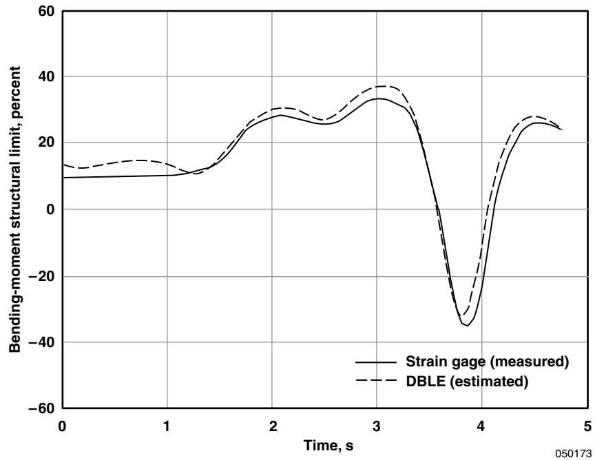
(a) Wing-root bending moment.
