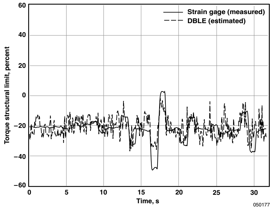
Figure 13. Wing-root torque doublet time history.
