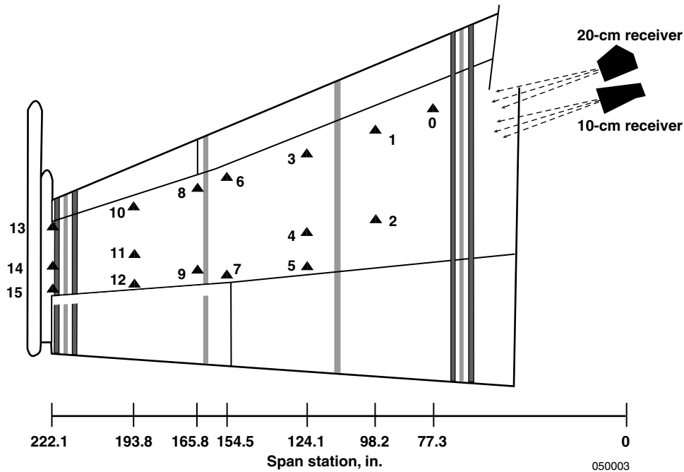
Figure 5. String potentiometer and flight deflection measurement system target placement illustration.
