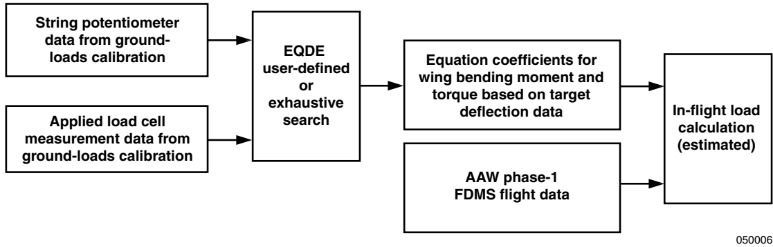
Figure 8. Deflection-based load equation development process flow chart.
