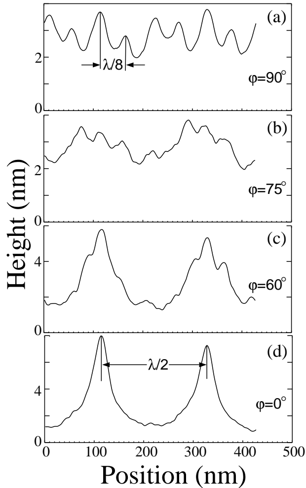
Figure 2 Band-averaged atomic force linescans of Cr deposited on Si wafer in the presence of a lin \triangle lin optical field, shown as a function of the angle \phi between the linear polarizations of the two counterpropagating travelling waves. The value of \phi are (a) 90^\circ (b) 75^\circ (c) 60^\circ and (d) 0^\circ . The vertical scale is set by the calibration of the atomic force microscope (accurate to \pm 10\% ), with the zero determined by measuring the height of a step formed by etching the sample. The zero is further corrected for a background of other isotopes (16%) and loss to Cr metastable ^5D states (estimated 7%).
