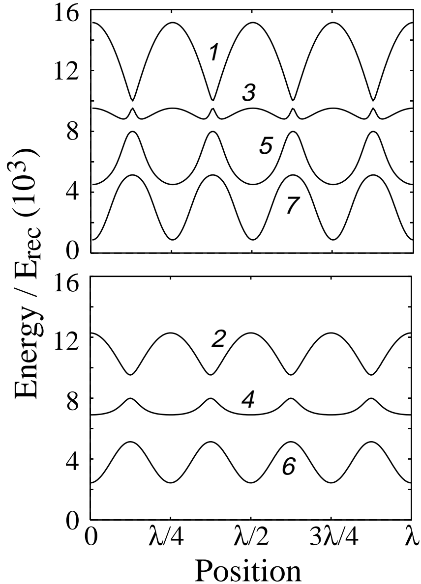
Figure 1 Adiabatic potentials in units of E_{\text{rec}} \equiv \hbar\omega_{\text{rec}} ( \omega_{\text{rec}} is the recoil frequency, which is 22 KHz) for the J_g=3 \rightarrow J_e=4 transition in Cr, for an optical field consisting of two linear orthogonally-polarized travelling waves with a Rabi frequency of \Omega=4.8 \times 10^4 \omega_{\text{rec}} and a detuning of \Delta=2.310^4 \omega_{\text{rec}} . (top) odd M -state family of potentials, (bottom) even M -state family of potentials. The potentials are numbered 1-7 for reference in the text.
