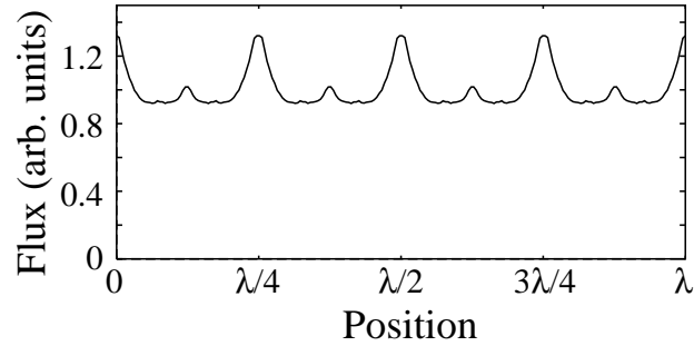
Figure 4 Quantum Monte Carlo calculation of the spatial distribution of Cr atoms traversing a lin \perp lin optical field, showing clear \lambda/8 features. All salient features of the experiment are taken into account, including a Gaussian laser profile with waist 65 \mu\text{m} ( 1/e^2 ), a peak Rabi frequency of \Omega=7.0 \times 10^4 \omega_{\text{rec}} , and a detuning of \Delta=2.3 \times 10^4 \omega_{\text{rec}} , ( \omega_{\text{rec}} is the recoil frequency for Cr, which is 22 kHz). Initial conditions include magnetic-level relative population weights of 0.5 ( M=+3,-3 ), 0.35 ( M=+2,-2 ), 0.1 ( M=+1,-1 ) and 0.05 ( M=0 ), a Gaussian transverse velocity distribution with rms spread of 7 \text{ m/s} and a Maxwellian longitudinal velocity distribution corresponding to a temperature of 1650 \text{ }^\circ\text{C} .
