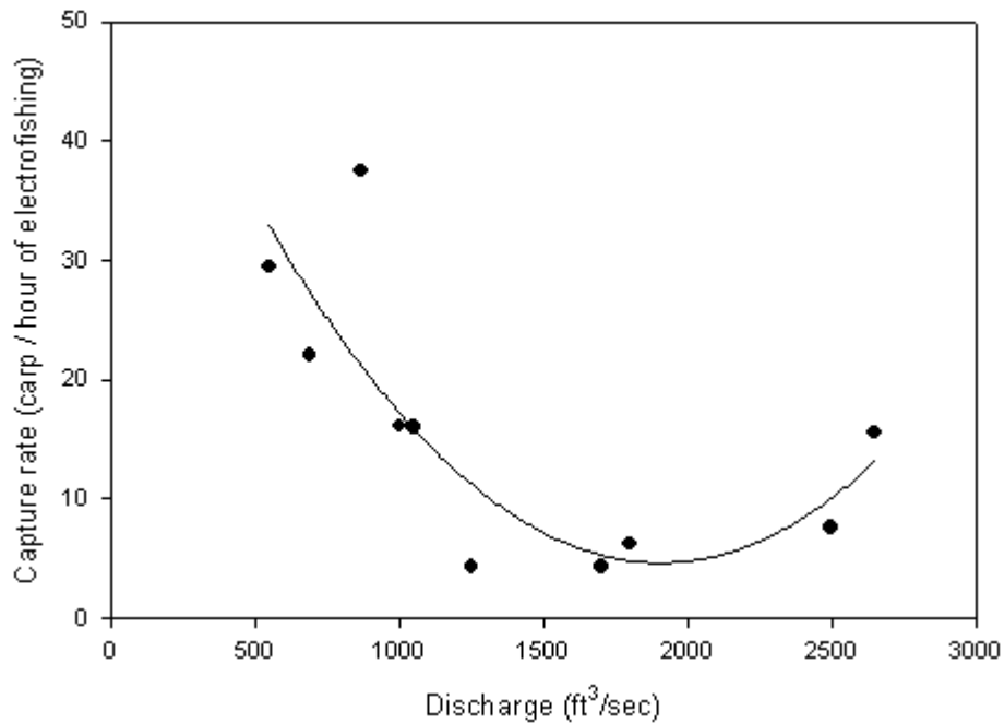
Figure 16. Significant negative correlation observed ( r = -0.733 ; p = 0.016 ) between discharge and capture rates of common carp collected in the San Juan River from PNM Weir to Hogback Diversion, 2001.
