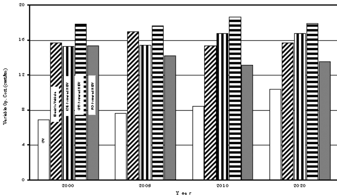
FIGURE 5. Variable Operating Costs, Including Battery Replacement Costs and Matching the Mean Range Requirements
