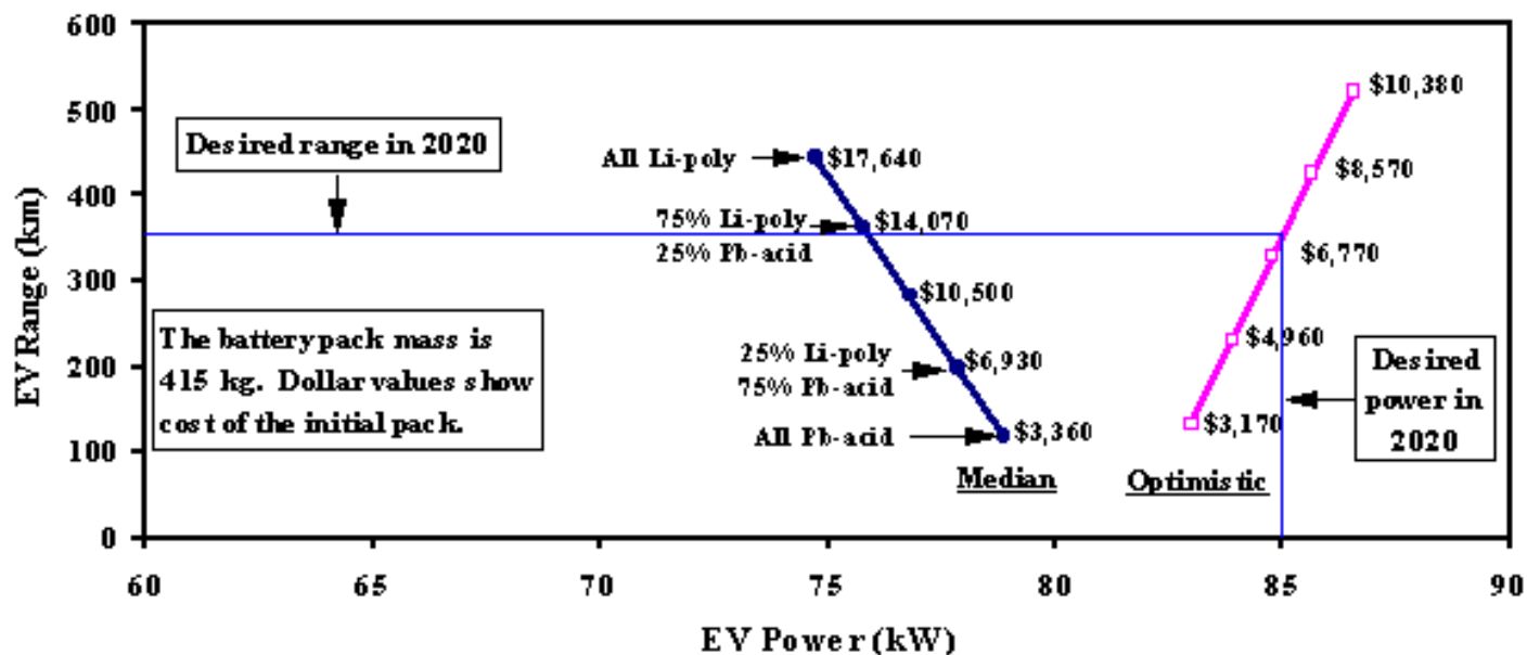
FIGURE 2. Analysis of Combined Lead-Acid and Lithium-Polymer Battery Packs for EV in 2020
