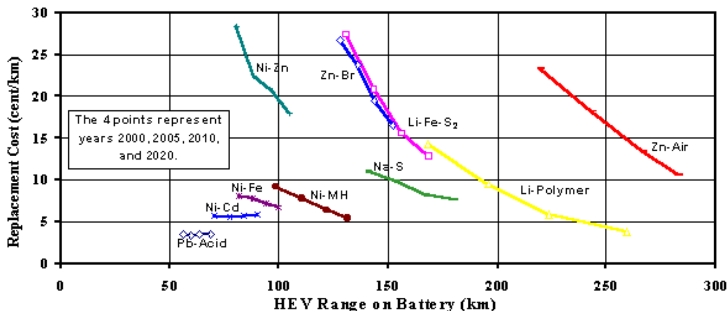
FIGURE 4. HEV Battery Replacement Cost and Range Associated with Half the Mean Power Requirements
