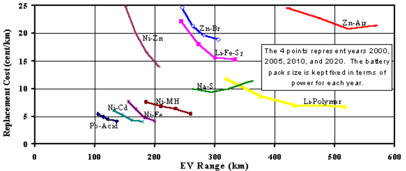
FIGURE 1. EV Battery Replacement Cost and Range Associated with the Mean Power Requirements
