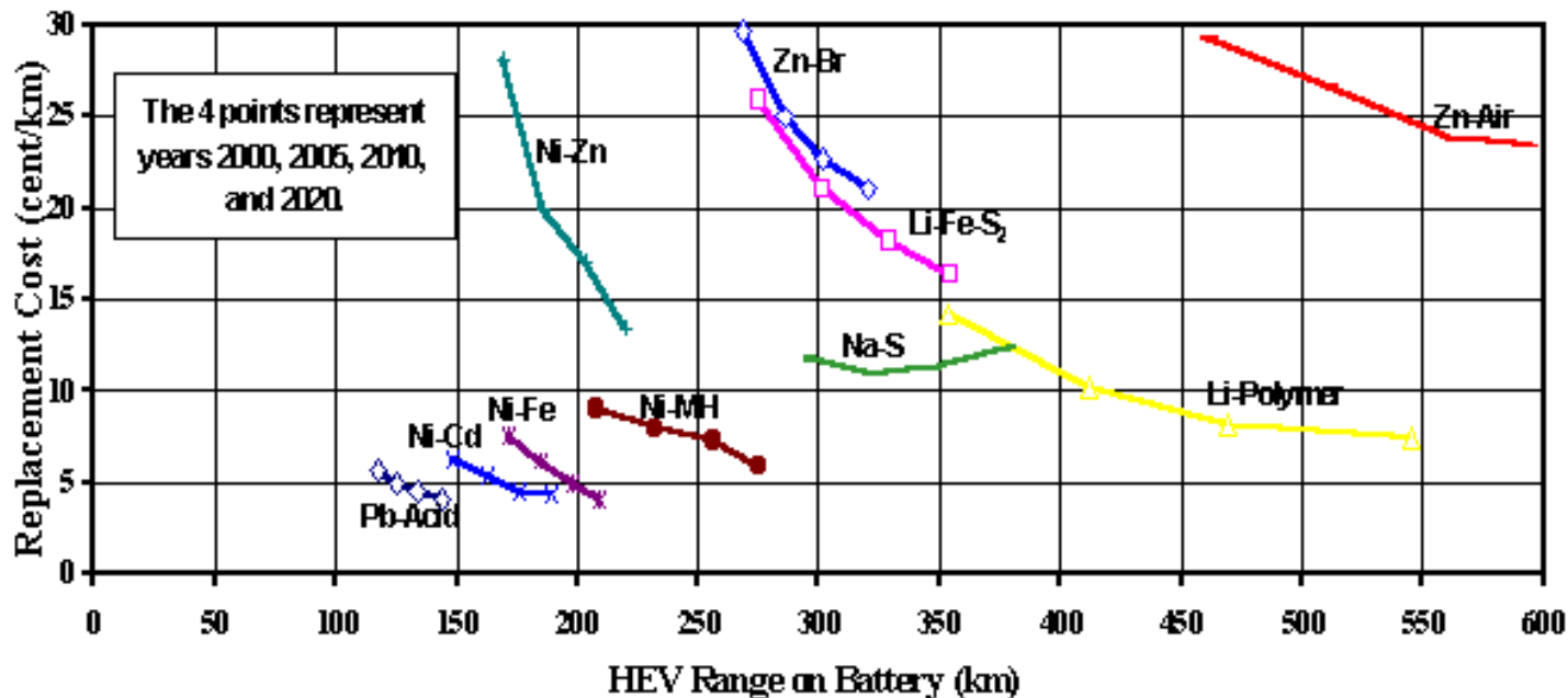
FIGURE 3. HEV Battery Replacement Cost and Range Associated with the Mean Power Requirements
