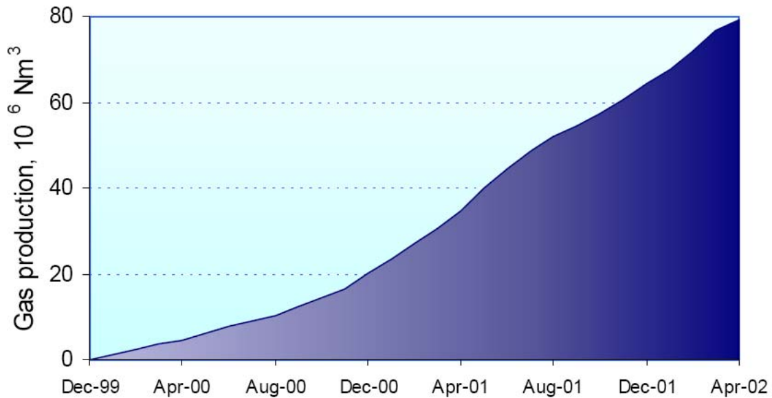
Figure 3-11: Gas production history at Chinchilla (Blinderman, 2003).
