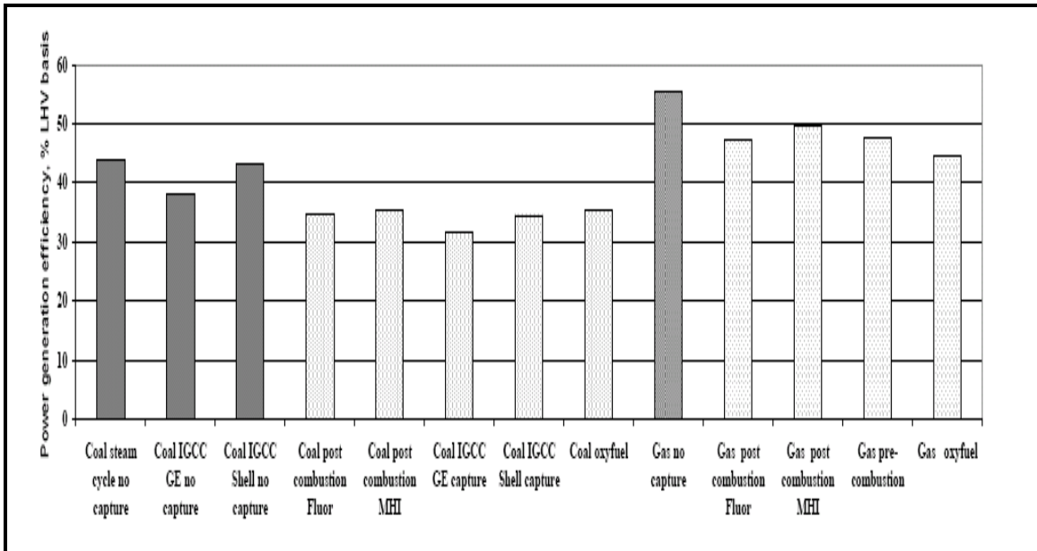
Figure 6-1: Thermal efficiencies of power plants with and without CO 2 capture, % LHV-basis (From Thambimithu, et al., 2005, and references therein: Davison 2005, IEA GHG 2004, IEA GHG 2003; 5 IEA GHG, 2000b; Dillon et al. , 2005).
