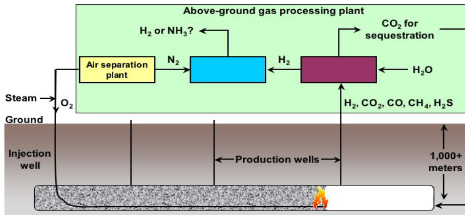
Figure 4-1: Schematic of the CRIP Process.
