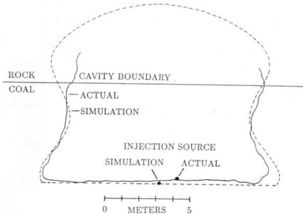
Figure 3-9: Comparison of actual and calculated cavity shapes in the plane perpendicular to the injection borehole at the injection point of the PSC CRIP cavity (Britten, 1986, 1987; Britten and Thorsness, 1988).
