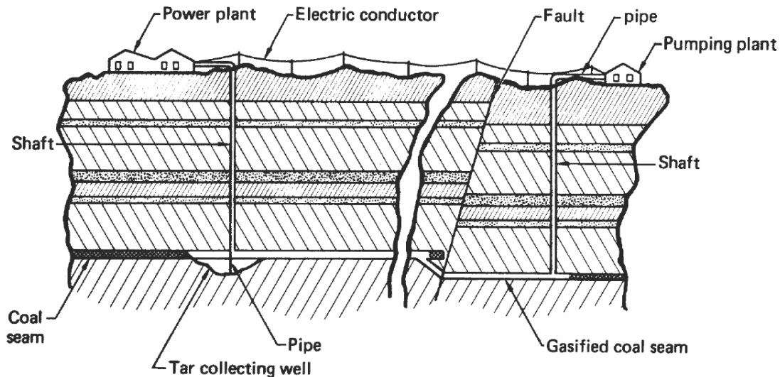
Figure 3-2: Reproduction of Betts's patent specifications, including an air, and ,if required, steam injection pipe from the pumping plant, in-situ gasification of the coal seam, and a collection pipe that feeds produced gas directly to an electric power plant (Olness and Gregg, 1977)
