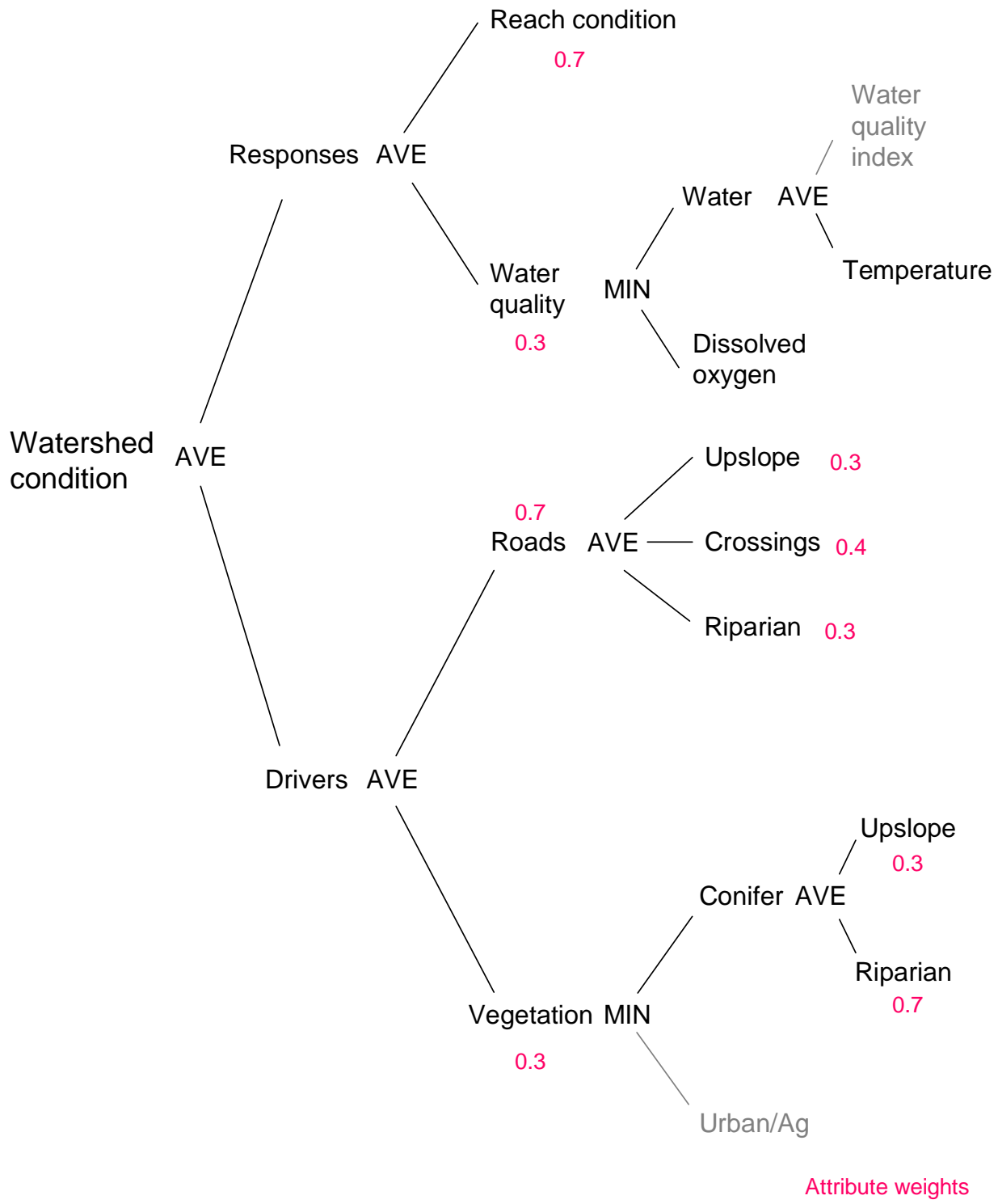
Figure 5. Graphical depiction of the watershed model structure for the West Cascades Province. The right-most nodes in the diagram represent watershed attributes that are evaluated and given an evaluation score. Evaluation scores are aggregated using the operators and weights depicted on the diagram to calculate an overall watershed condition score.
