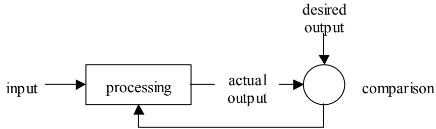
FIGURE 2. SUPERVISED TRAINING
