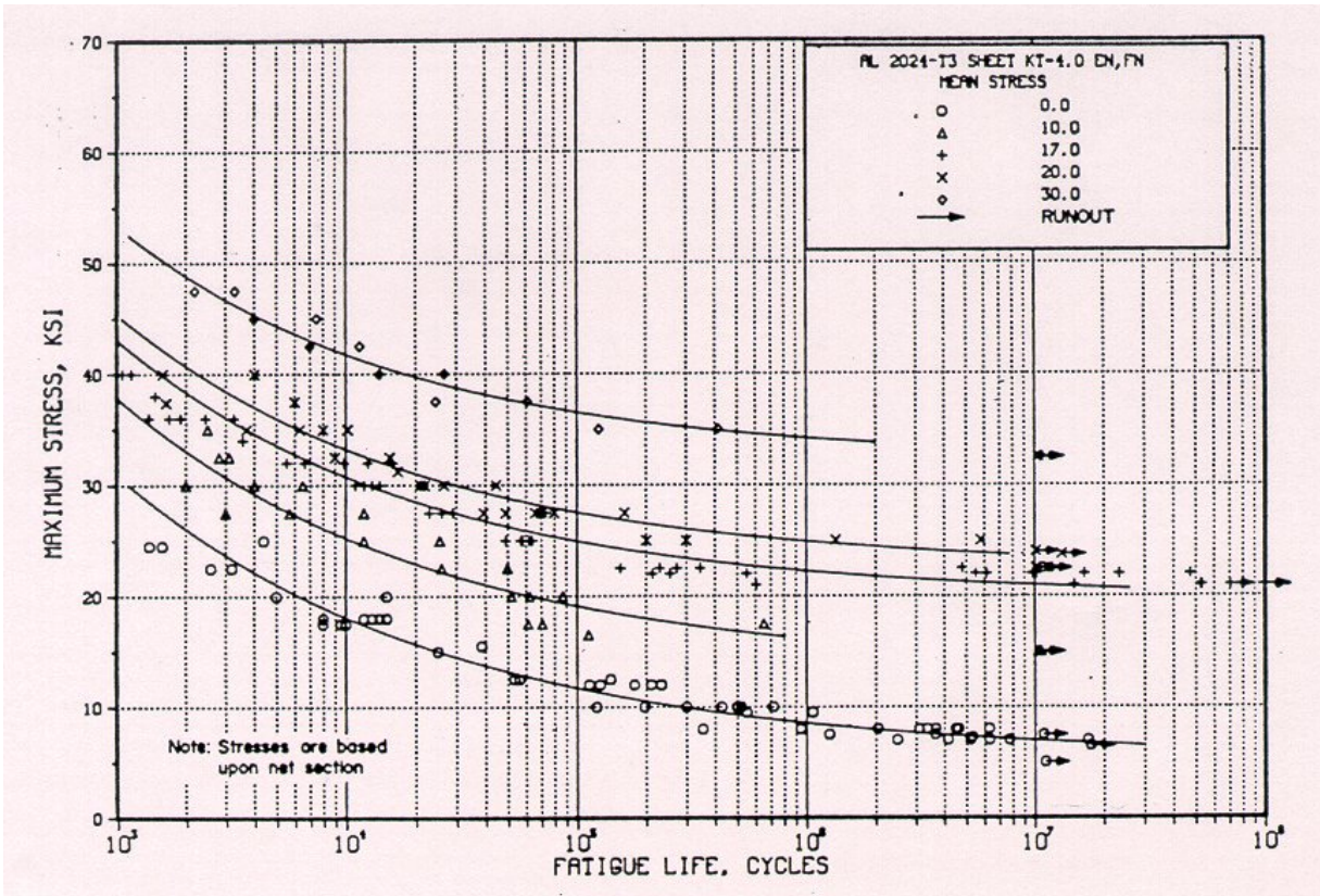
FIGURE 9. S-N CURVE OF AN AL 2024-T3 SHEET
