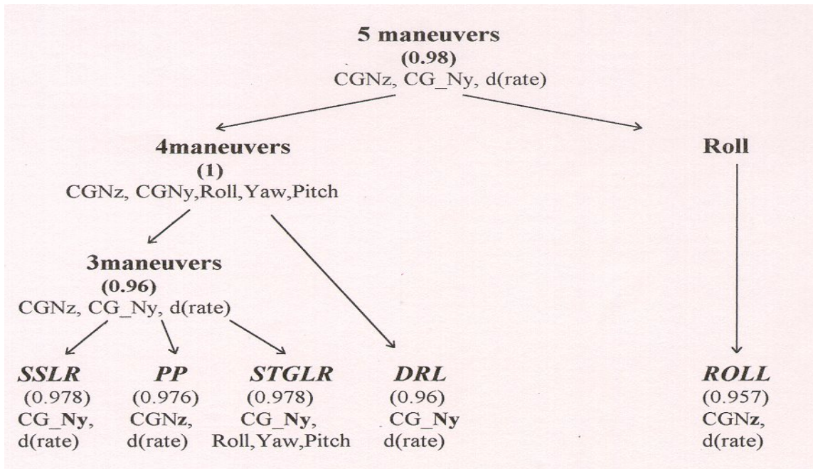
FIGURE 13. CLASSIFICATION ALGORITHM
