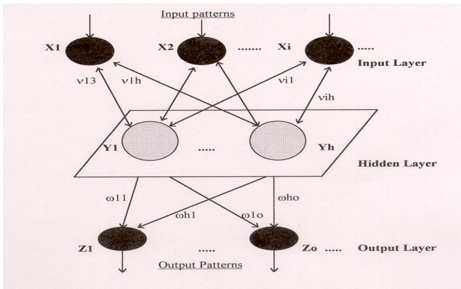
FIGURE 3. BACKPROPAGATION NEURAL NETWORKS, FULLY INTERCONNECTED
