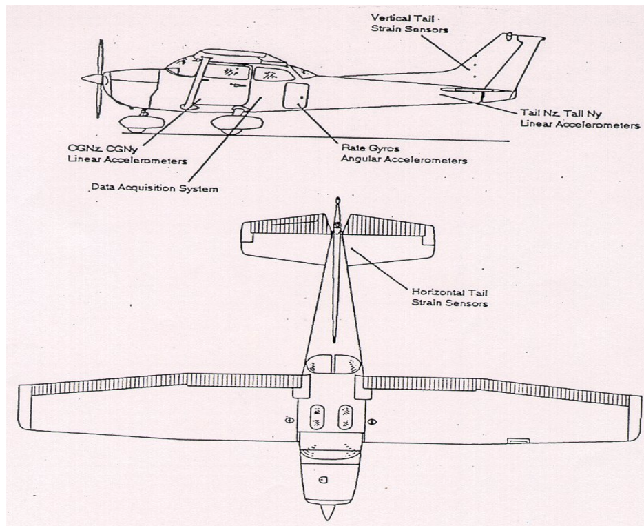
FIGURE 8. INSTRUMENTATION SETUP
