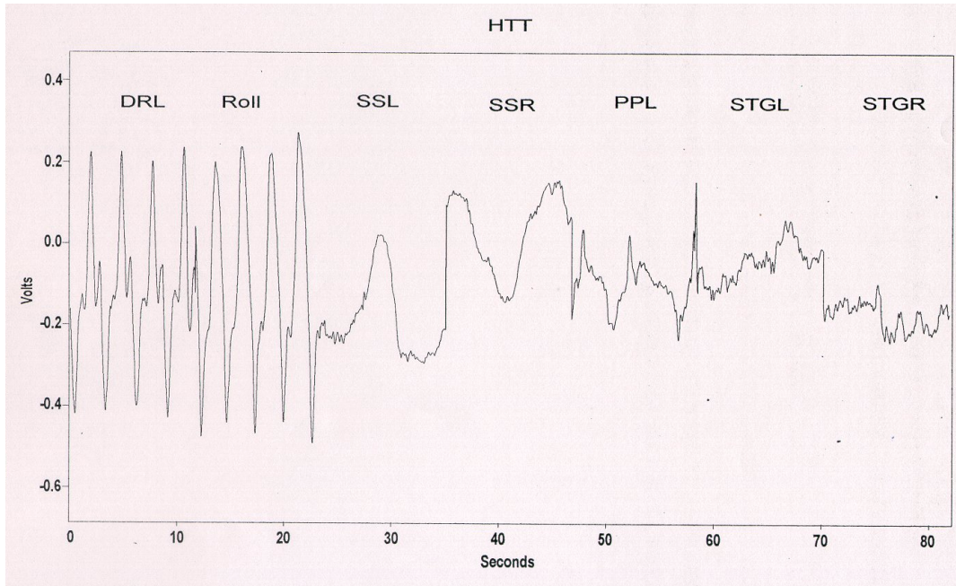
FIGURE 10. HORIZONTAL TAIL LOAD DURING MANEUVERS
