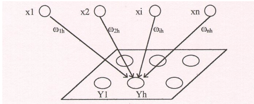
FIGURE 6. CONNECTIONS FROM THE INPUT LAYER TO A HIDDEN PE Y_h
