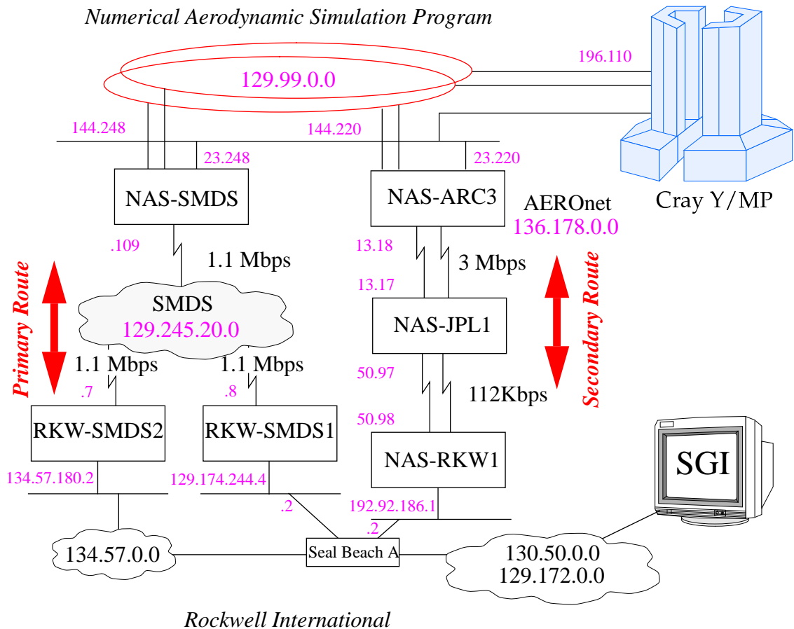
FIGURE 1. SMDS Testbed
