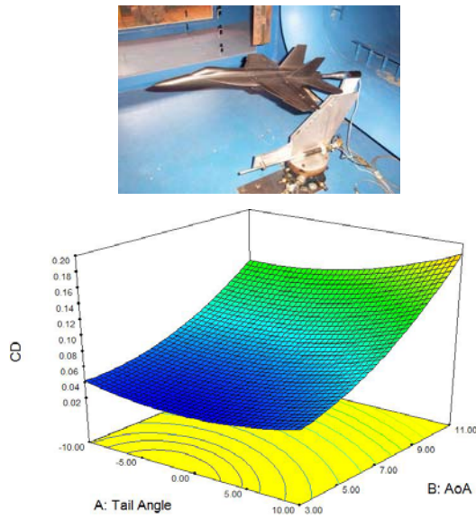
Fig. 1. Drag Coefficient Response Surface.
