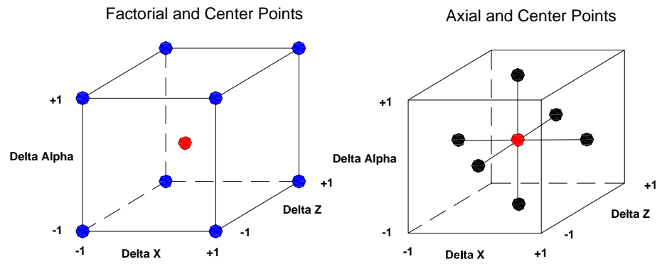
(a) face-centered design (cuboidal CCD)
