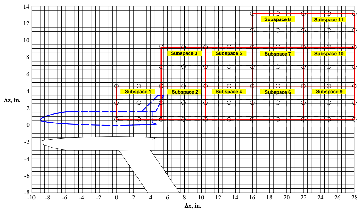
Fig. 7. Partitioning of the overall inference space for the LBGG stage separation experiment.
