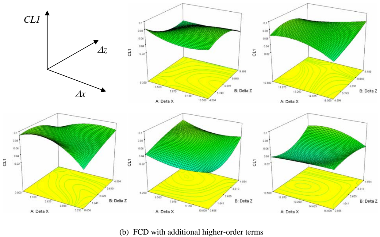
Fig. 13. Comparison of Lift Coefficient Response Surfaces in Subspaces 1-5 from Simplified FCD and FCD with additional higher-order terms; \Delta\alpha = 2.5 degrees.
