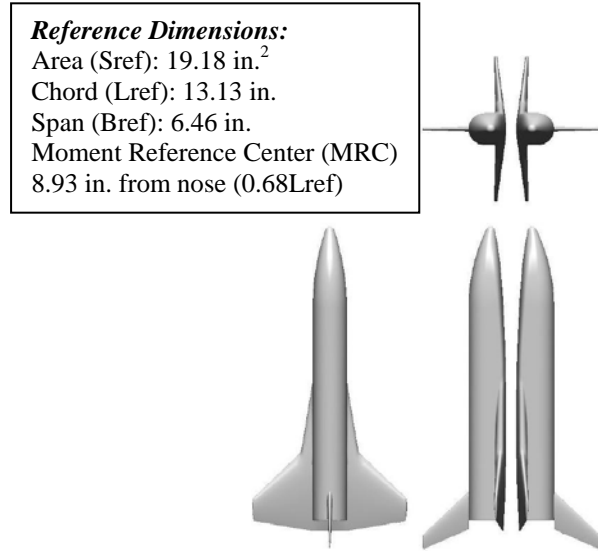
Fig. 2. LGBB bimese wing-body configuration in belly-to-belly arrangement.
