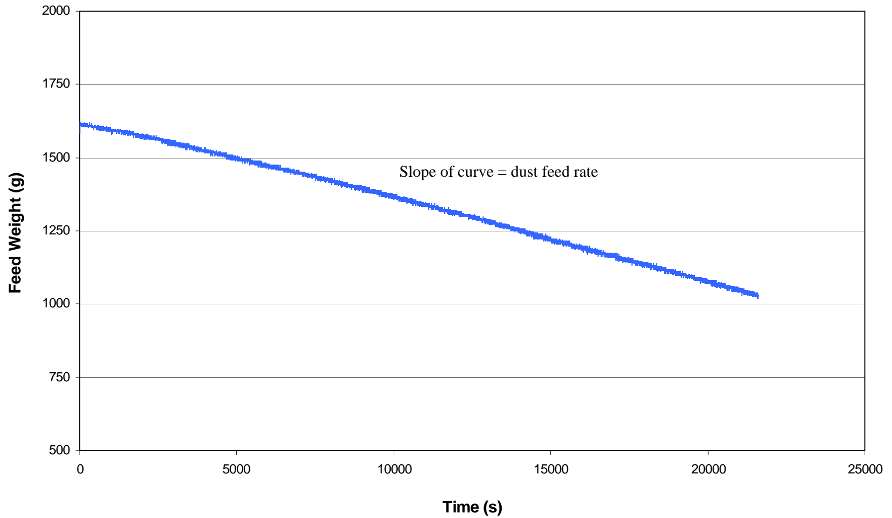
Figure C-5. Change in Pural NF dust scale reading with time during performance test run V001B-3.
