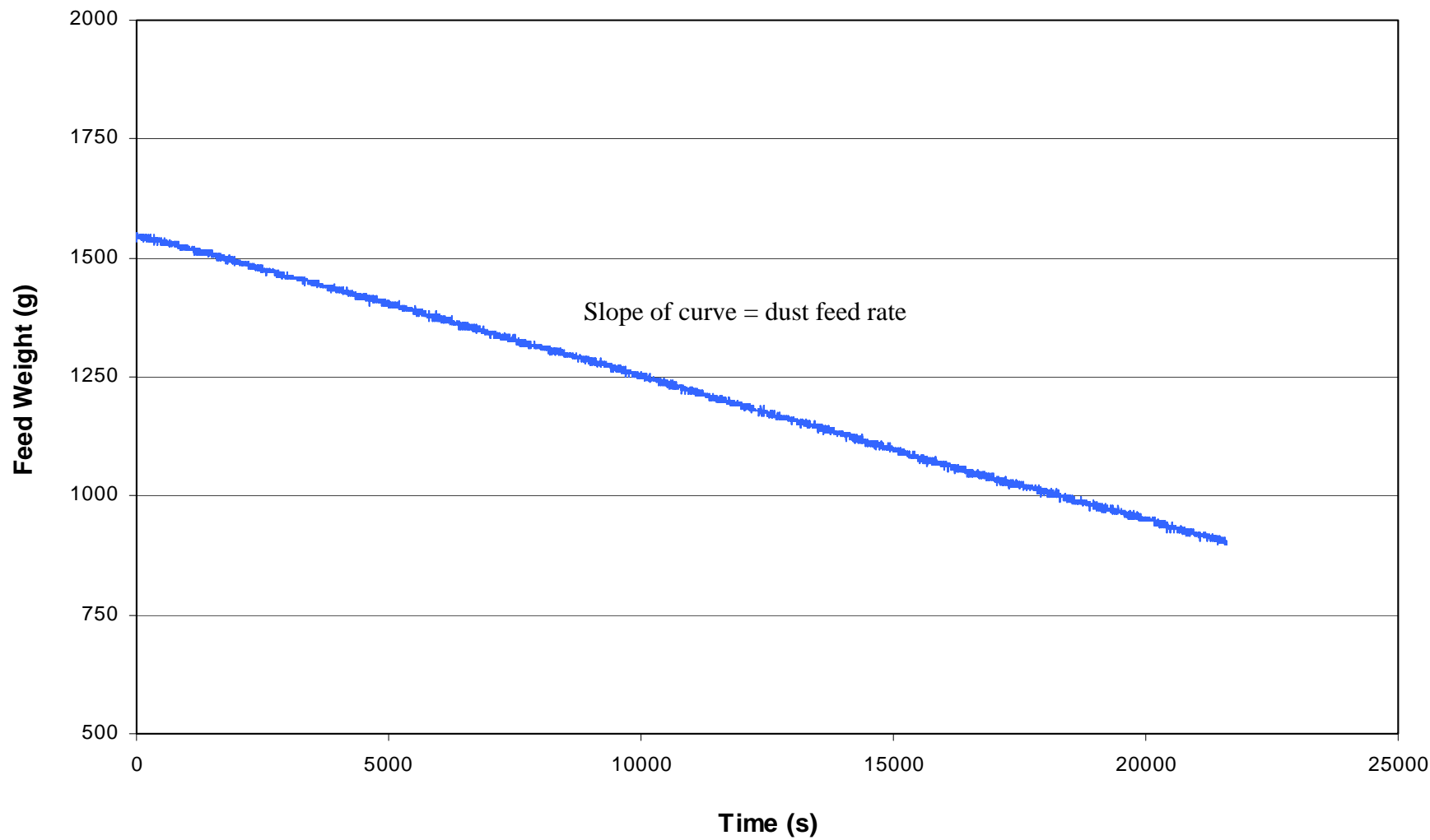
Figure C-1. Change in Pural NF dust scale reading with time during performance test run V001B-1.
