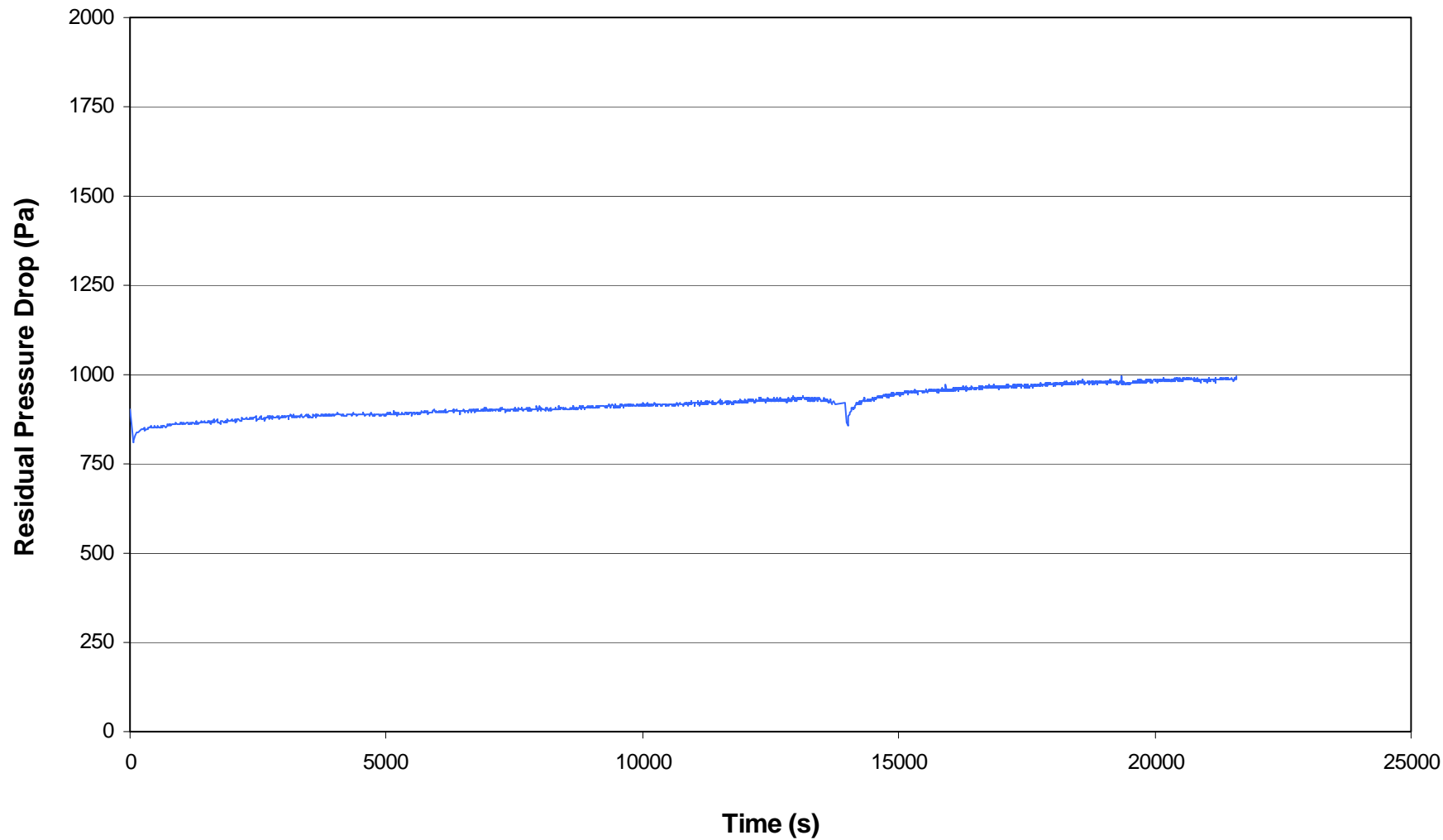
Figure C-4. Residual pressure drop across filter fabric during performance test run V001B-2.
