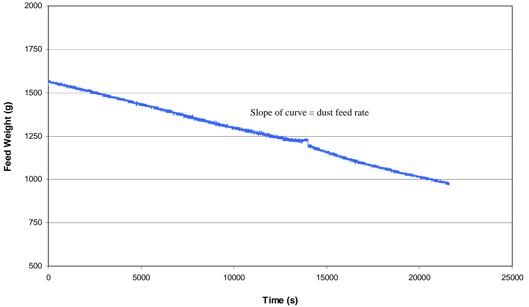
Figure C-3. Change in Pural NF dust scale with time during performance test run V001B-2.
