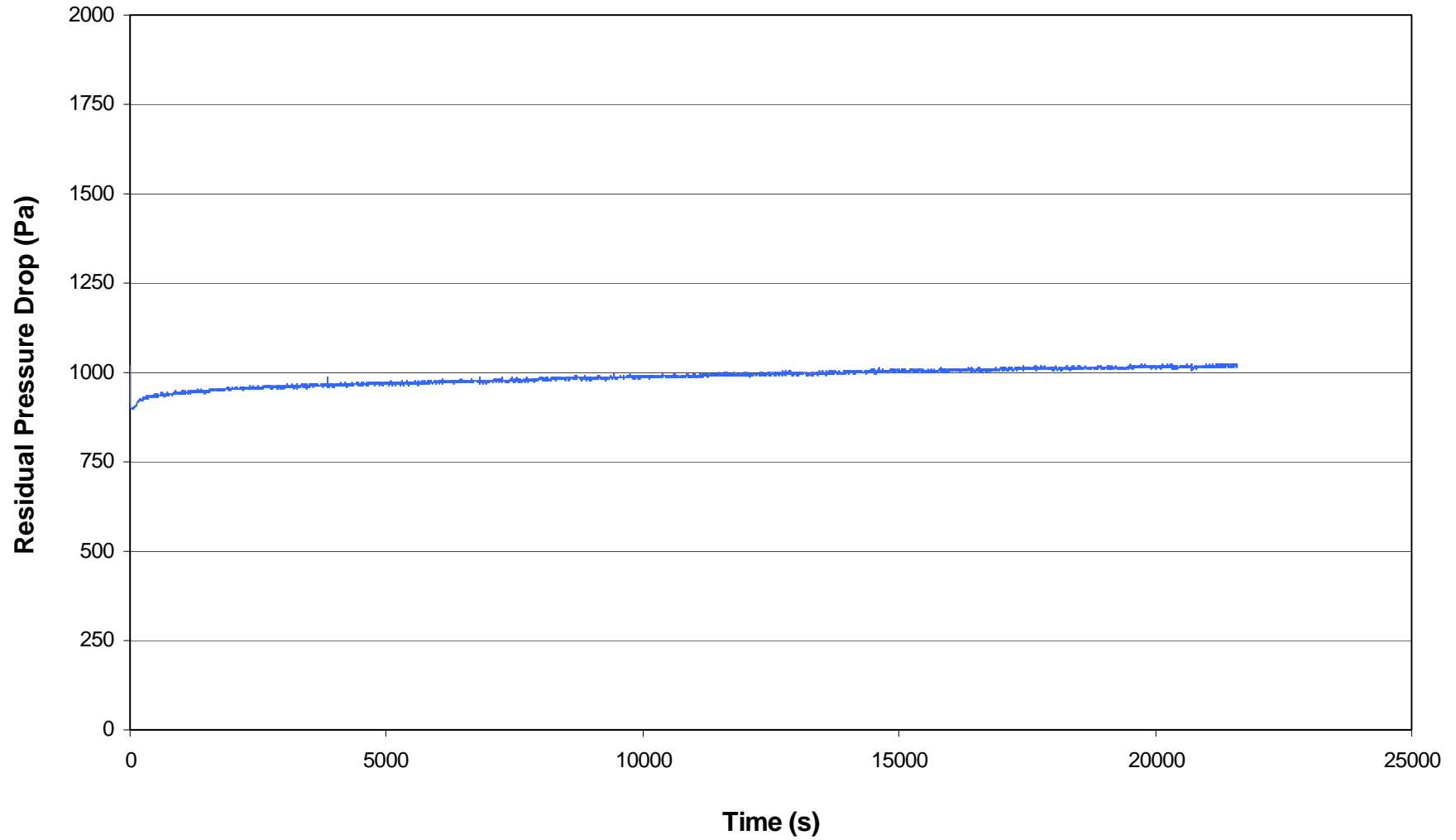
Figure C-6. Residual pressure drop across filter fabric during performance test run V001B-3.
