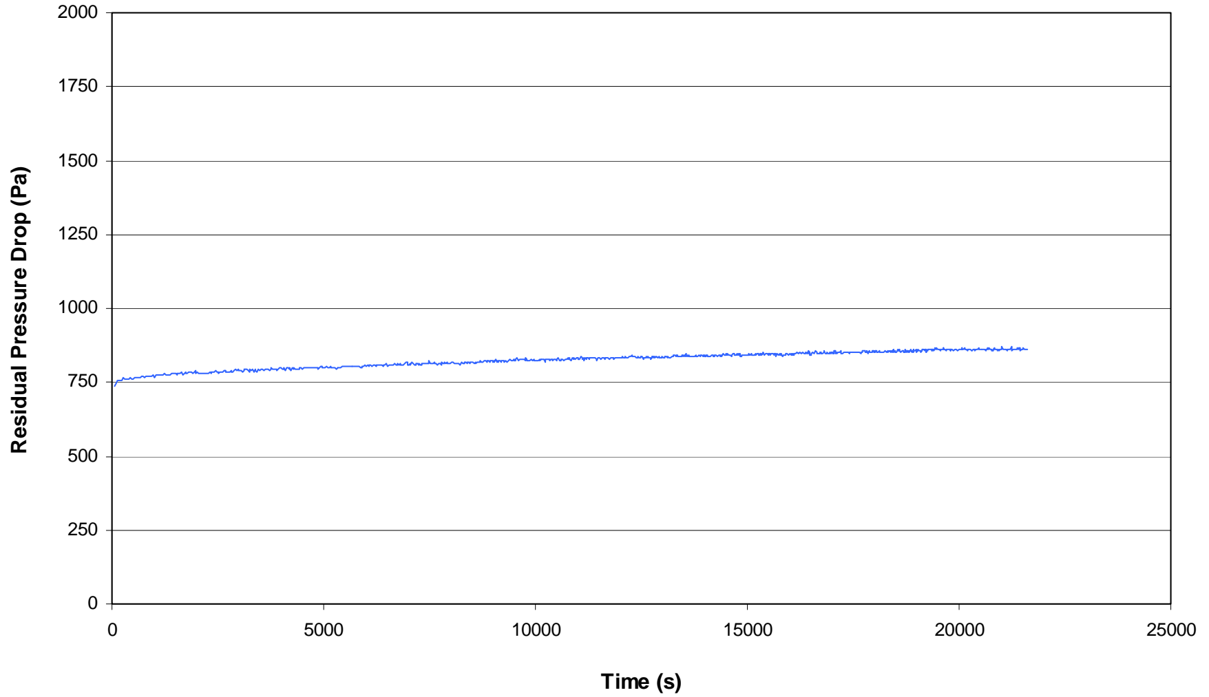
Figure C-2. Residual pressure drop across filter fabric during performance test run V001B-1.
