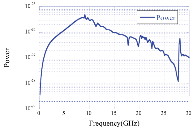
Fig. 13. Power spectrum of D01 type electrode.
