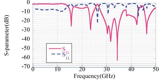
Fig. 5 Simulated S-parameter of KEKB-FB button electrode.
