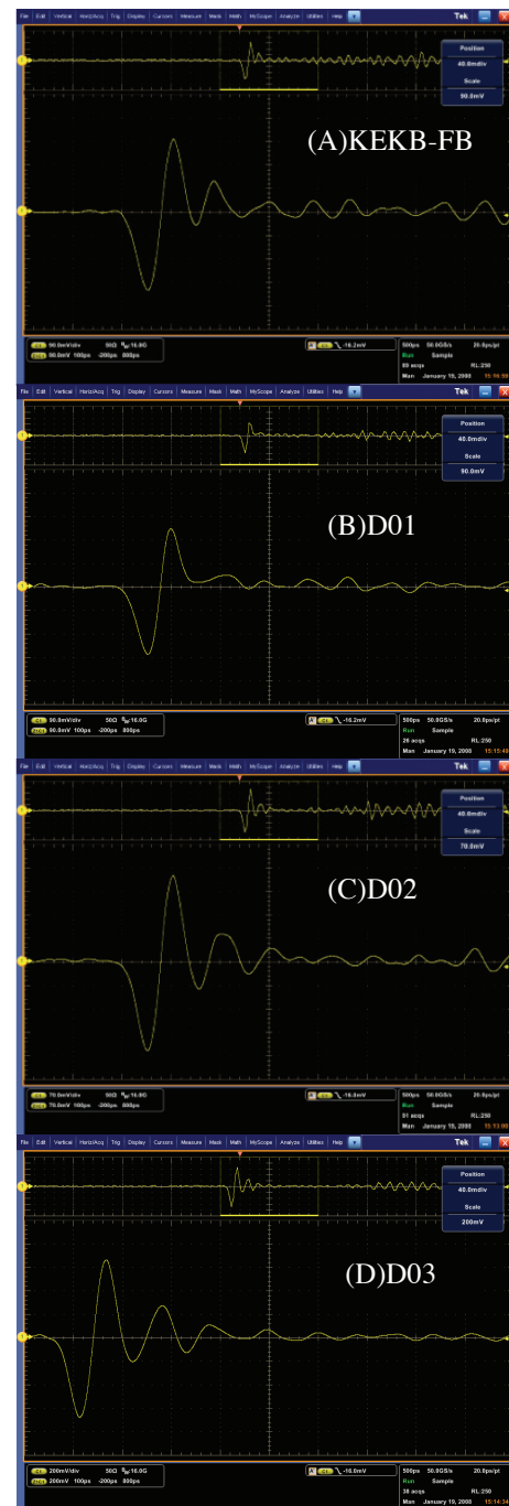
Fig. 19. Beam response of BPMs from linac beam.
