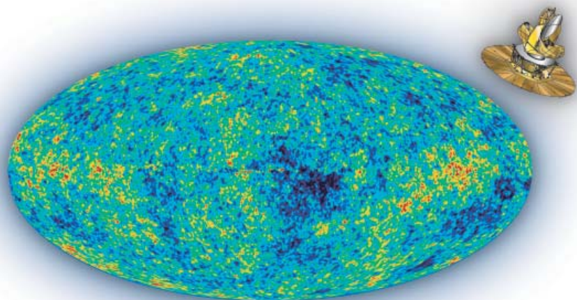
The map of the cosmic microwave background, the afterglow of the Big Bang, obtained by NASA’s Wilkinson Microwave Anisotropy Probe (WMAP).
