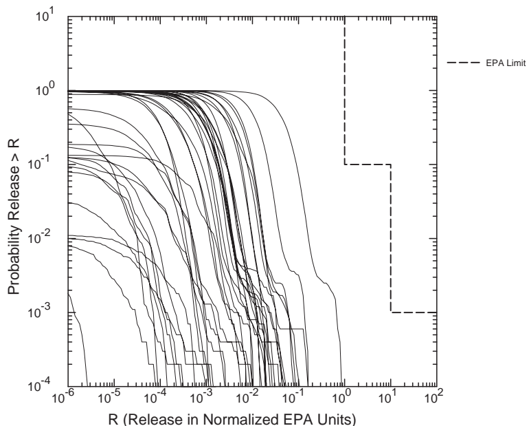
Figure 2. Spallings Releases Calculated Using the Average Radioactivity of 3 Randomly Sampled CH-TRU Waste Streams
