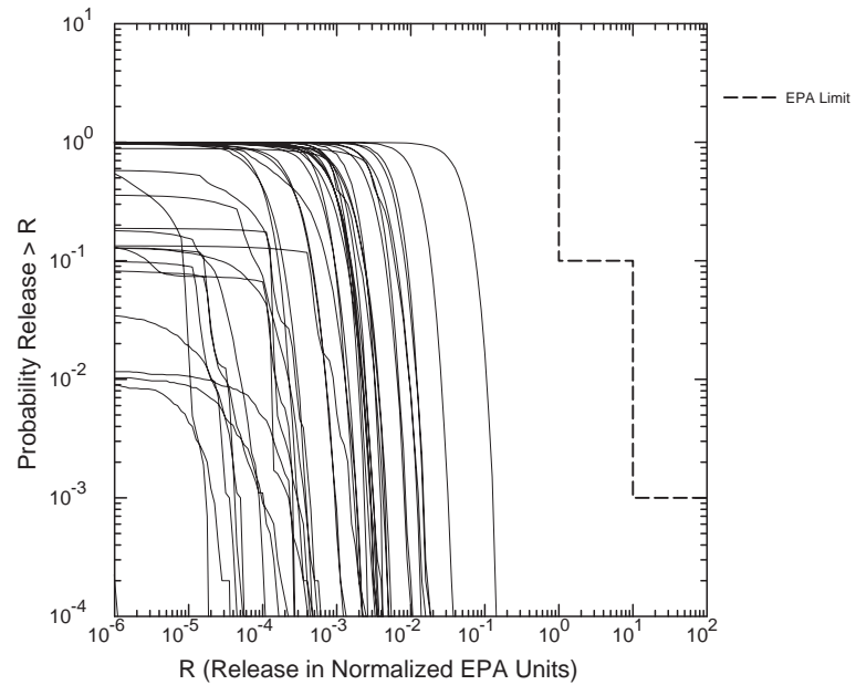
Figure 1. Spallings Releases Calculated Using the Average Radioactivity Over All CH-TRU Waste Streams
