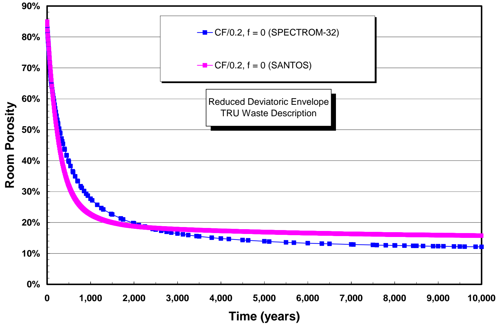
Figure 2. Comparison of SANTOS and SPECTROM-32 Room Porosity Results for a TRU Waste Reduced Deviatoric Envelope and No Gas Generation.
