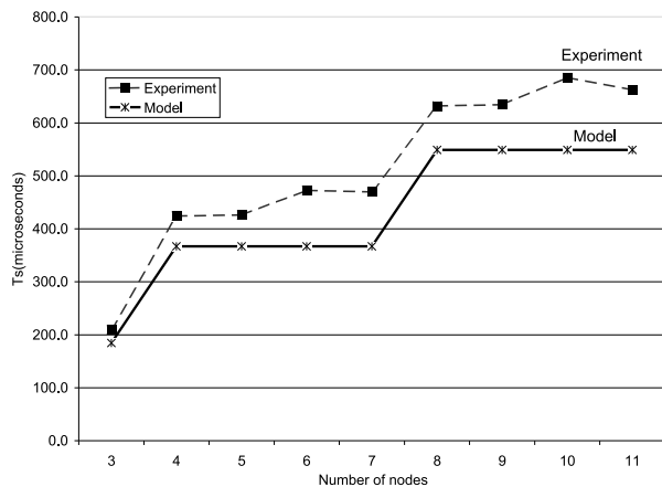
Figure 6: Stabilization Time ( T_s ) over TCP
