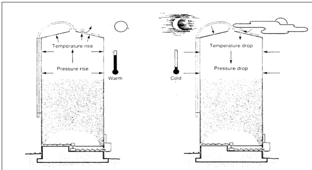
Diagram 5. Oxygen-limiting silos must “breathe” to compensate for temperature and pressure changes
