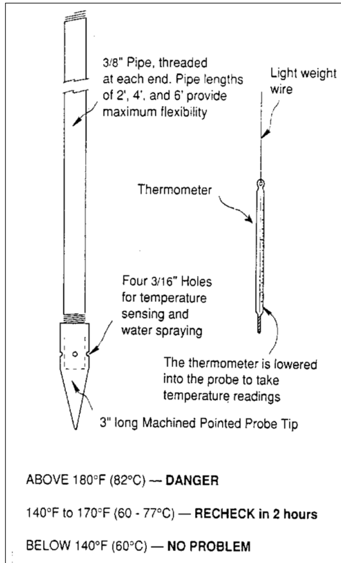
Diagram 9. Temperature Probe
