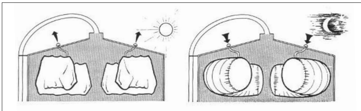
Diagram 6. "Breather Bag" system in oxygen-limited silo
