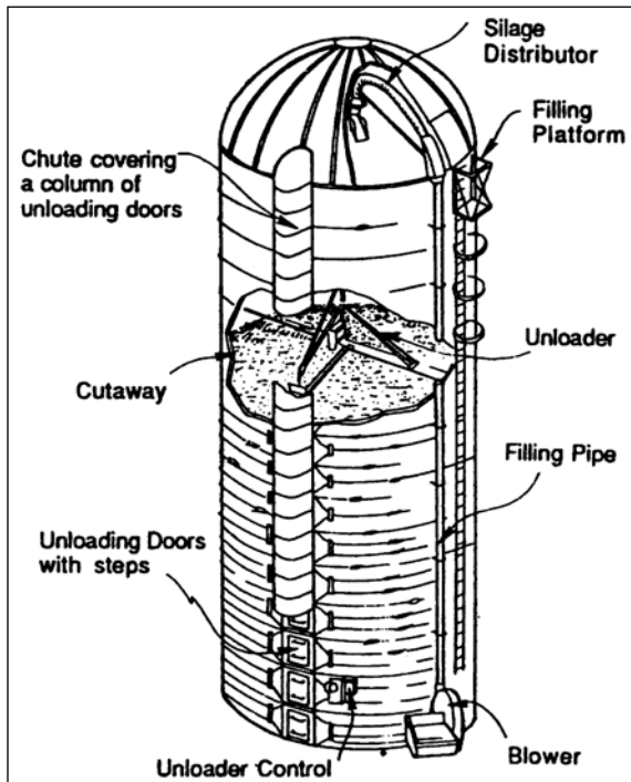
Diagram 2. Features of Conventional Vertical Silo
