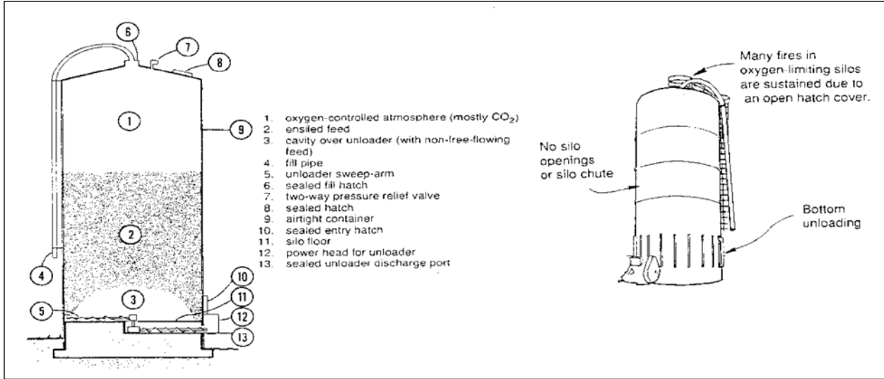
Diagram 3 and 4. Features of an oxygen-limiting silo
