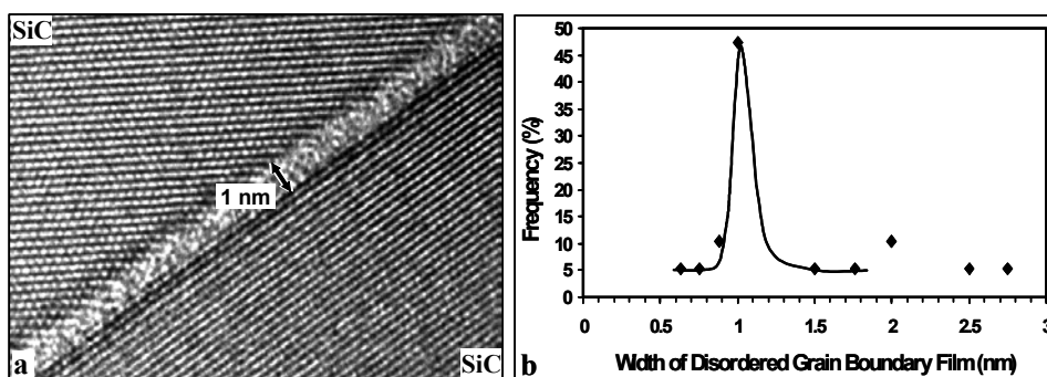
Fig. 2: (a) High-resolution electron micrograph showing a typical intergranular film between two SiC matrix grains. An amorphous structure is observed with a width of about 1 nm. (b) Distribution of amorphous grain-boundary widths determined by high-resolution electron microscopy. The grain-boundary width ranges from 0.75 nm to 2.75 nm, with a mean of about 1 nm.
