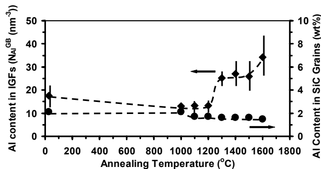
Fig. 6: Plots of EDS-determined Al site density in grain-boundary films ( N_{Al}^{GB} ) and in SiC matrix grains (Al/SiC, wt%) as a function of annealing temperature.
