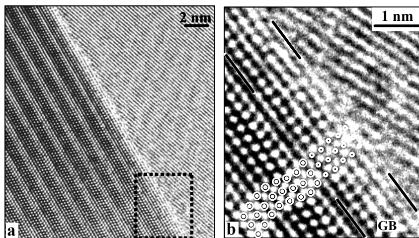
Fig. 3: (a) High-resolution electron microscopy image for a grain-boundary area in ABC-SiC annealed at 1200°C for 500 hrs. Amorphous intergranular film is crystallized. (b) Enlarged image from the framed area in (a). Atomic stacking in 6H-SiC grain on the bottom-left side is marked by black circles. 2H-wurtzite atomic stacking in grain-boundary film (GB) are marked by white circles. Note the epitaxial orientation relationships between the grain-boundary film and the 6H-SiC matrix grain.
