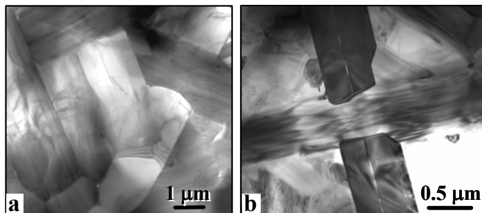
Fig. 1: (a) Bright-field TEM images showing elongated SiC grains in ABC-SiC, showing (b) the interlocked nature of the elongated grains.
