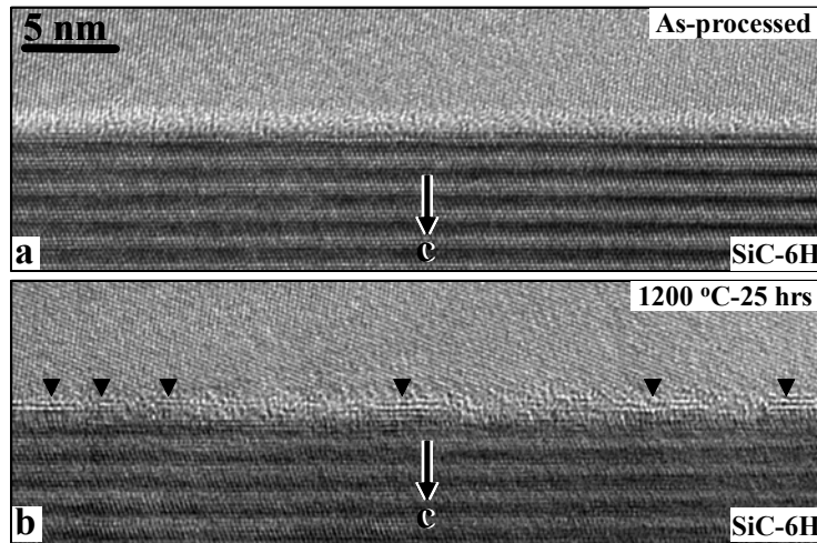
Fig. 4: (a) High-resolution image of an amorphous intergranular film in as-hot-pressed ABC-SiC. (b) The same film as in (a) but after in situ heating in a transmission electron microscope at 1200°C for 25 hrs. Arrowheads indicate the discrete, crystallized boundary segments.
