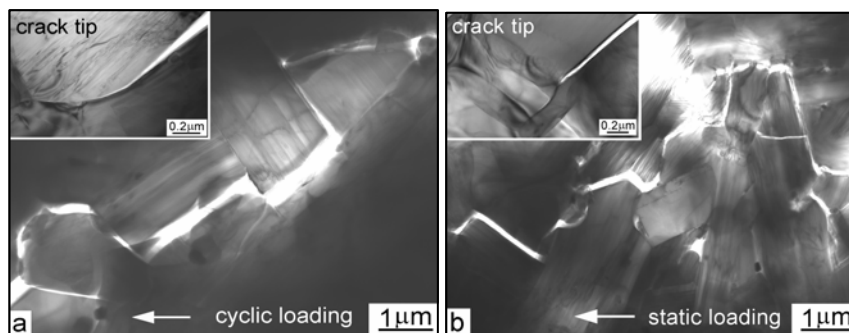
Fig. 8: TEM images of the intergranular crack profiles at the crack-tip in ABC-SiC at 1300°C under (a) cyclic loading (25 Hz, R = 0.1 ), and (b) static loading. Arrows indicate the direction of crack propagation. No evidence of viscous boundary layers or creep damage.
