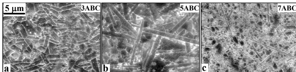
Fig. 9: Morphologies of the 3ABC-, 5ABC-, and 7ABC-SiC are shown in images in (a) to (c), respectively. Note the significant changes in dimension and area density of the elongated SiC grains. Note also the bimodal grain systems with 5ABC-SiC.
