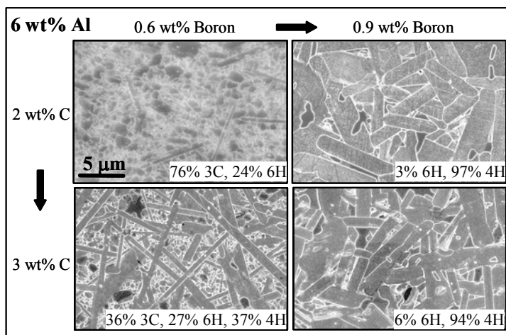
Fig. 10: Microstructural changes with fixed Al (6 wt%) and adjusted boron or carbon contents. Phase compositions are marked in each image. Effects of boron and carbon additions in changing microstructure and phase composition are clear.
