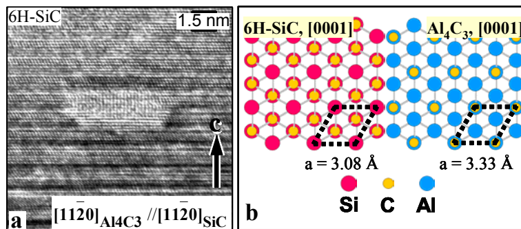
Fig. 5: (a) \text{Al}_4\text{C}_3 -based nanoprecipitate formed in a 6H-SiC grain annealed at 1400°C. The viewing directions are marked. (b) Atomic models for 6H-SiC and \text{Al}_4\text{C}_3 projected along the [0001] direction. The similarity between the two structures can be seen.
