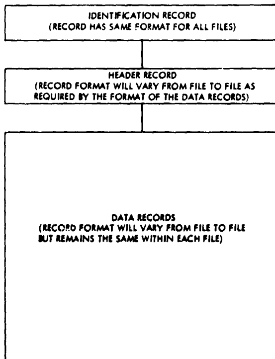
Fig. 4. File structure
