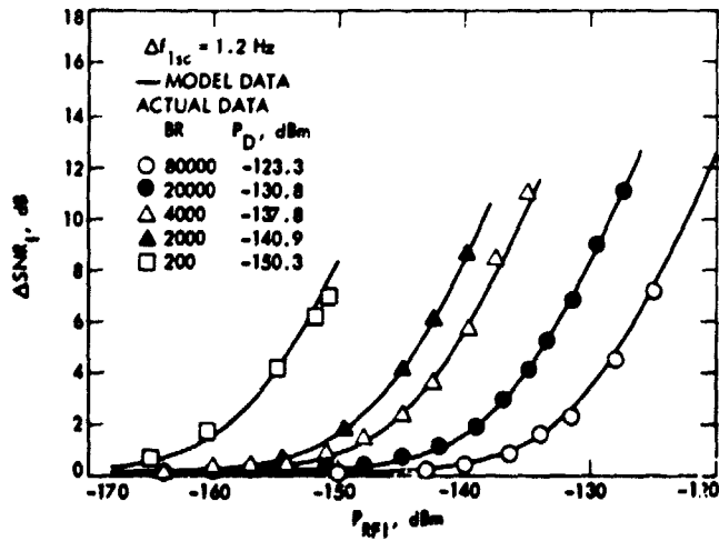
Fig. 4. \Delta SNR_I vs P_{RFI} for selected values of BR
