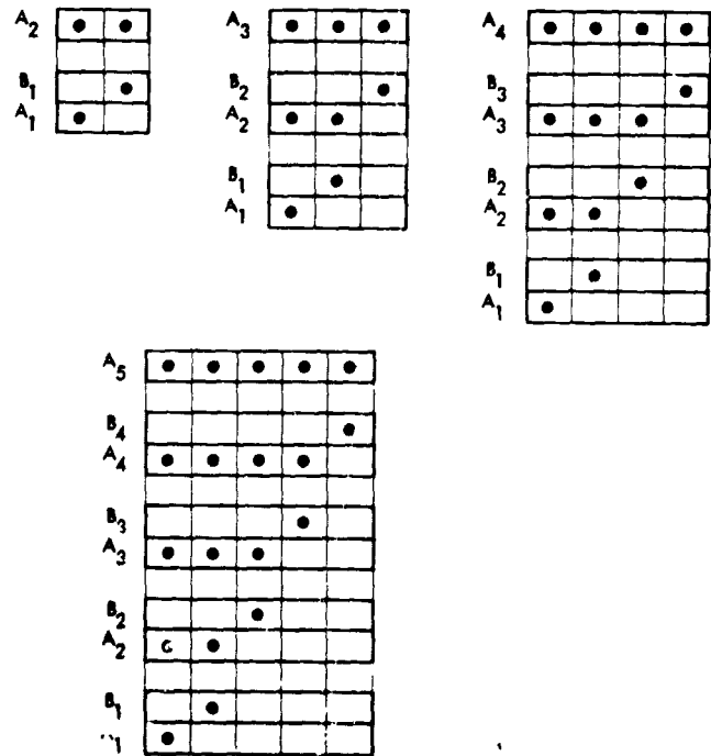
Fig. 3. Efficient priority codes that maximize the number of users on n wires, n = 2, 3, 4, 5
