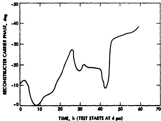
Fig. 9. Long-term stability test results on the Block III residual carrier loop's reconstructed carrier (modulation angle \theta = 90 deg, PN data, 100 kbps, data on 360 kHz square wave subcarrier, ST/N_0 = 4 dB)
