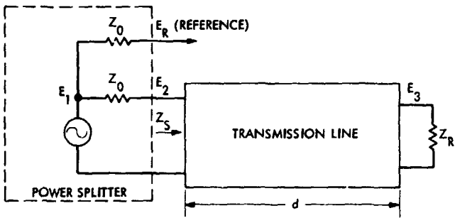
Fig. 1. Transmission line distribution system model
