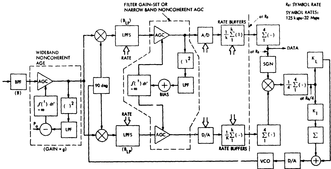
Fig. 1. Partial functional block diagram of the feasibility model, Multimegabit Demodulator/Detector Assembly
