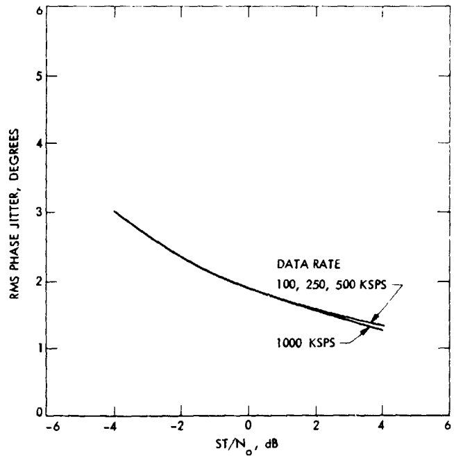
Fig. 10. Design values of Costas loop rms phase jitters as functions of ST/N_0
