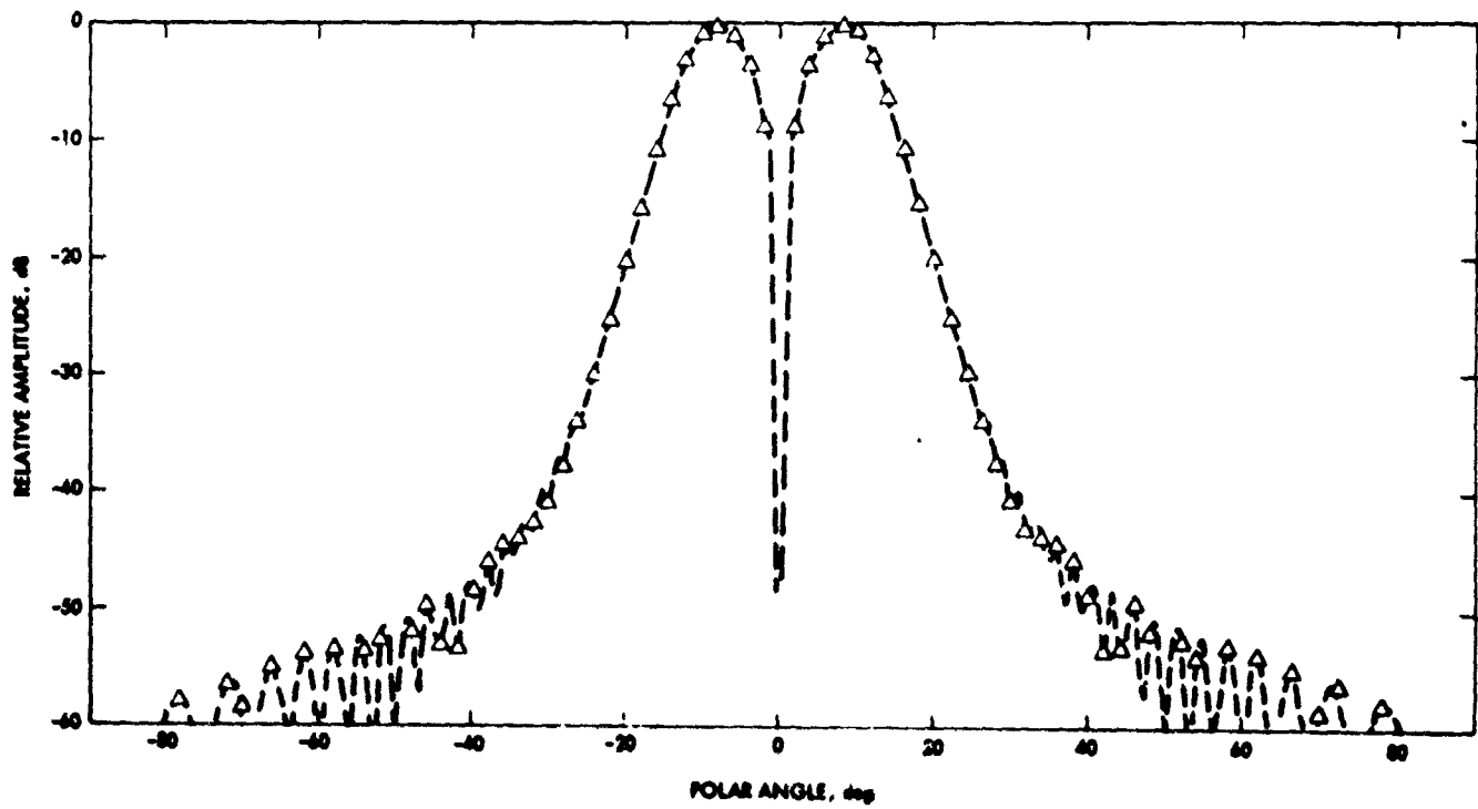
Fig. 7. Williams horn, EH 00 Mode, 8.415 GHz, E theta
