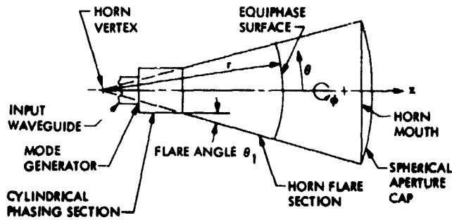
Fig. 1. Horn geometry
