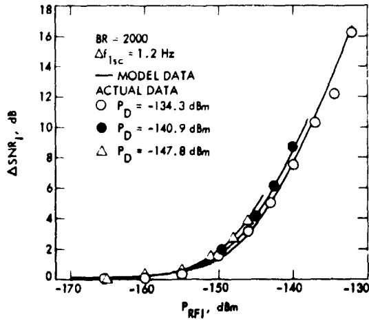
Fig. 3. \Delta SNR_I vs P_{RFI} for selected values of P_D
