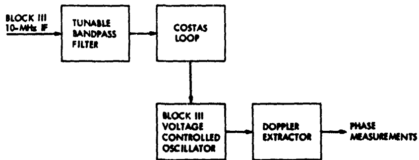
Fig. 11. Test configuration to simulate the effect of receiver front end asymmetric filtering on the phase shifts of the reconstructed carrier in the presence of Doppler shifts
