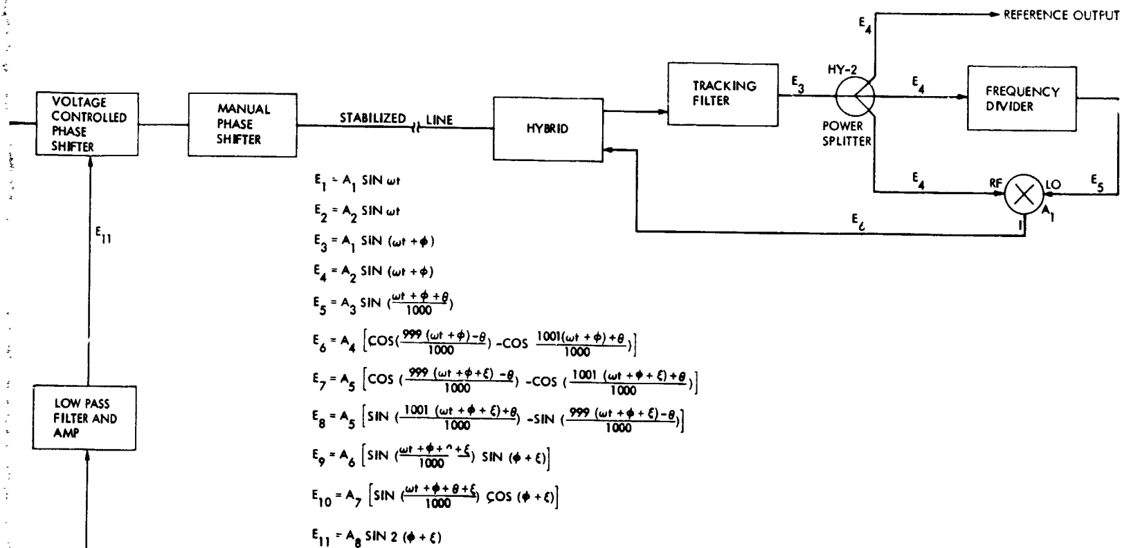
Fig. 2. Simplified block diagram of transmission line stabilizer
