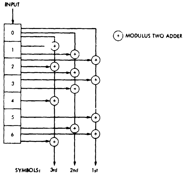
Fig. 2. Connection diagram of (7, 1/3) code
