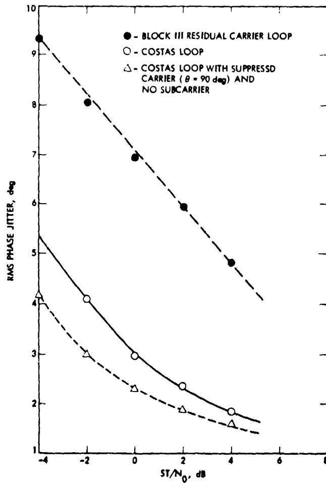
Fig. 10. Residual carrier signalling phase jitter measurements (data rate = 100 kbps, modulation angle \theta = 90 deg, subcarrier frequency = 360 kHz)
