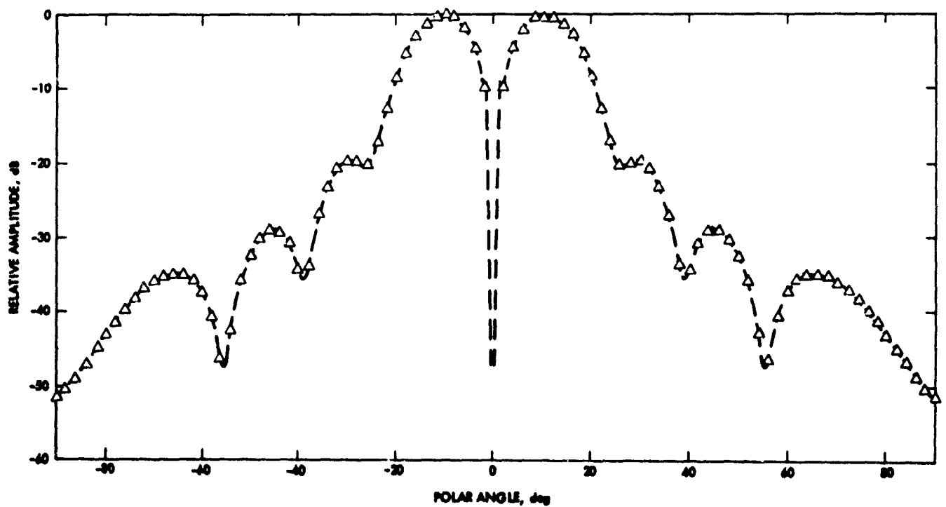
Fig. 3. Brunstein horn, EH 01 Mode, 8.415 GHz, E theta
