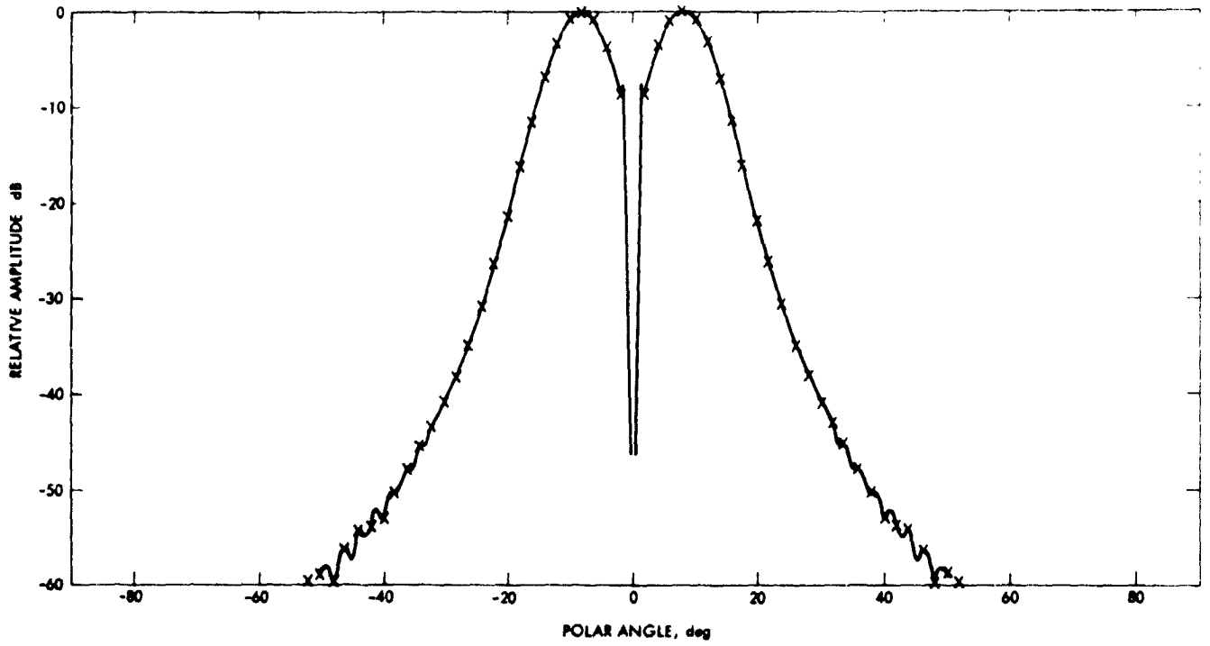
Fig. 8. Williams horn, TE_{01} Mode, 8.415 GHz, E phi
