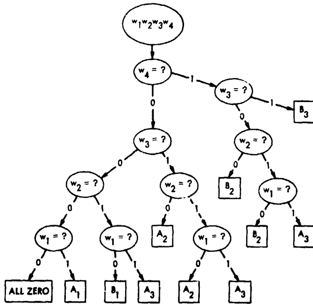
Fig. 2. Decision tree for decoding the example code given in Fig. 1.
