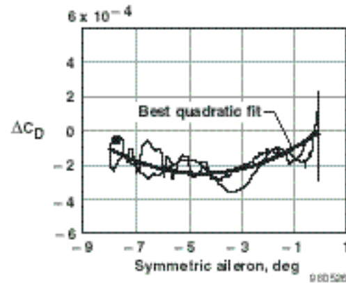
Figure 4. Variation of incremental drag with symmetric outboard aileron deflection for a one-sided raised-cosine maneuver (data filtered, period = 400 sec, \epsilon = 0.000076 ).
