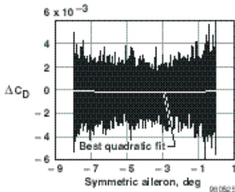
Figure 3. Variation of incremental drag with symmetric outboard aileron deflection for a one-sided raised-cosine maneuver (no filtering, period = 400 sec, \epsilon = 0.0012 ).
