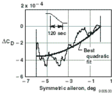
Figure 8. Variation of incremental drag with symmetric outboard aileron deflection for a ramp maneuver (data filtered, peak-to-peak excitation period = 120 sec, = 0.000093).
