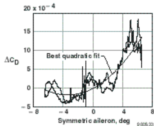
Figure 11. Variation of incremental drag with symmetric outboard aileron deflection for a real-time adaptive configuration optimization maneuver; results obtained in real time (data filtered, period = 200 sec, = 0.00032).
