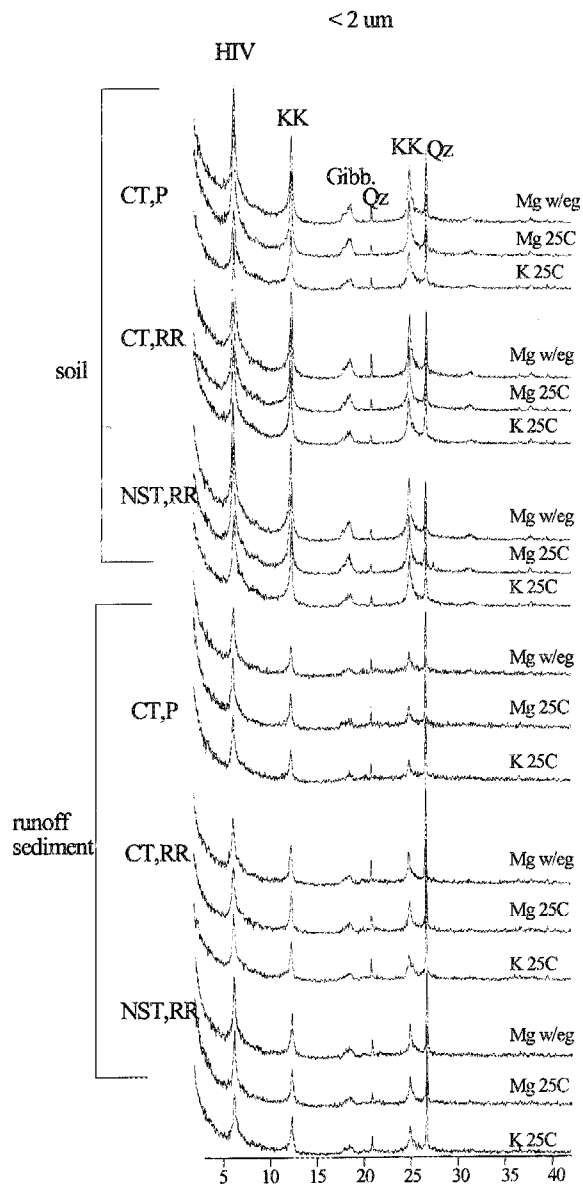
Fig. 3. X-ray diffractograms of clay fractions for soil and sediment for three plots (CT-P, CT-RR, and NST-RR). KK: kaolinite, gibb: gibbsite and qz: quartz. Mg w/eg is Mg-saturated with ethylene glycol solvation, and Mg and K 25°C are Mg- and K-saturated analyzed at 25°C.
