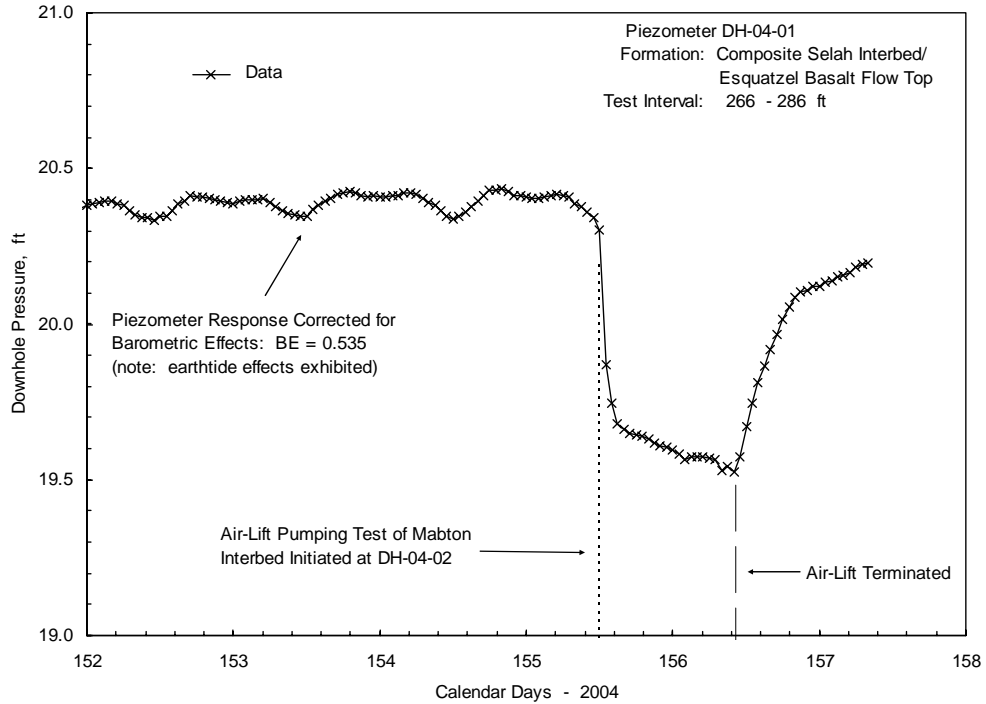
Figure 7. Piezometer DH-04-01 Baseline Monitoring Response Indicating Cross-Formational Leakage During Air-Lift Pumping Test of the Mabton Interbed at Test Well DH-04-02 (from Spane, 2004)
