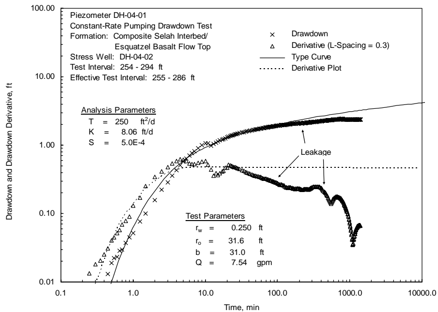
Figure 6. Type-Curve and Derivative Plot Analysis of Constant-Rate Pumping Test Drawdown Data for Piezometer DH-04-01: Test Interval 254 - 294 ft. (from Spane, 2004)
