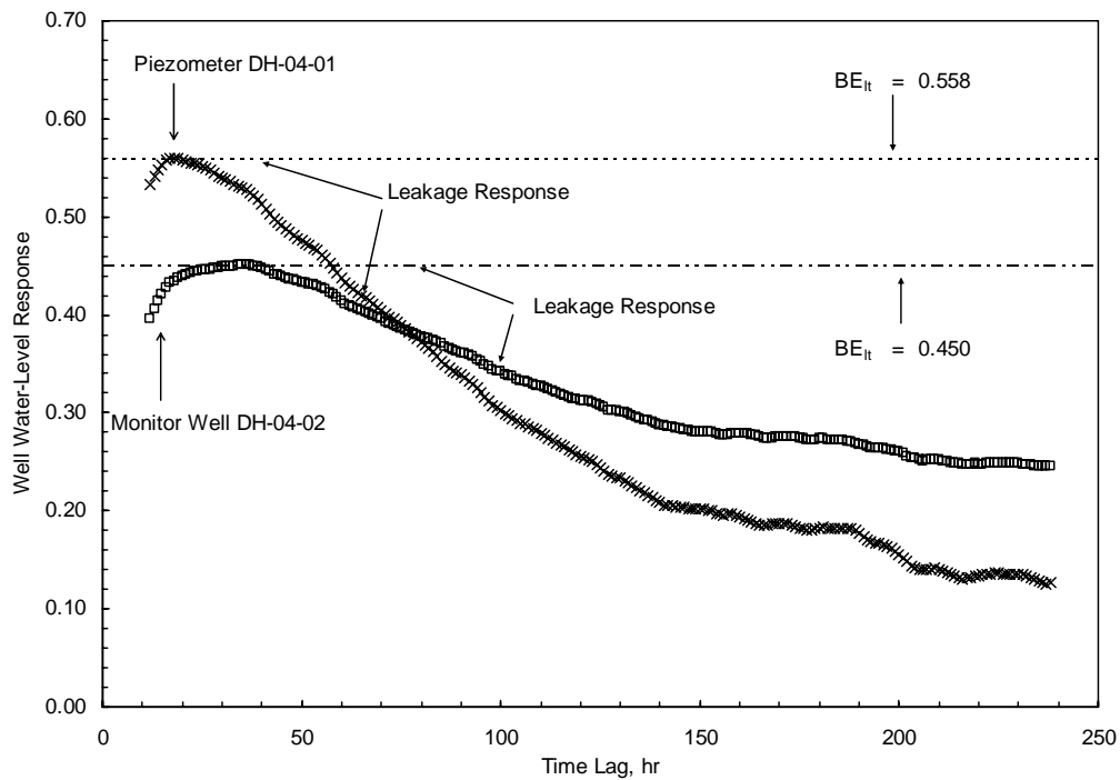
Figure 8. Comparison of DH-04-01 and DH-04-02 Barometric Response Plots (from Spane, 2004)
