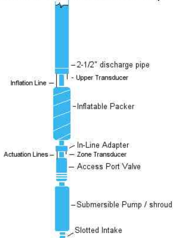
Figure 3. Packer assembly for hydrologic borehole tests.
