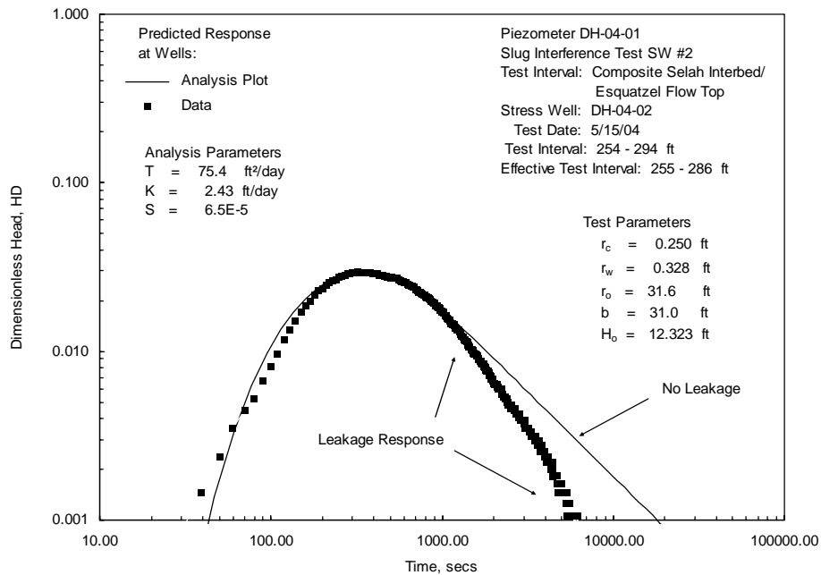
Figure 5. Type-Curve Analysis Plot for Slug Withdrawal Interference for Piezometer DH-04-01: Composite Selah Interbed/Esquatzel Basalt Flow Top (from Spane, 2004)
