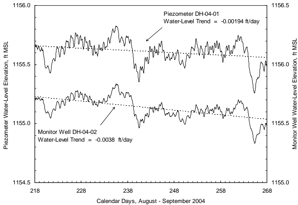
Figure 9. Comparison of Baseline Water Level Fluctuations for DH-04-01 and DH-04-02, August 5 – September 24, 2004 (from Spane, 2004)
