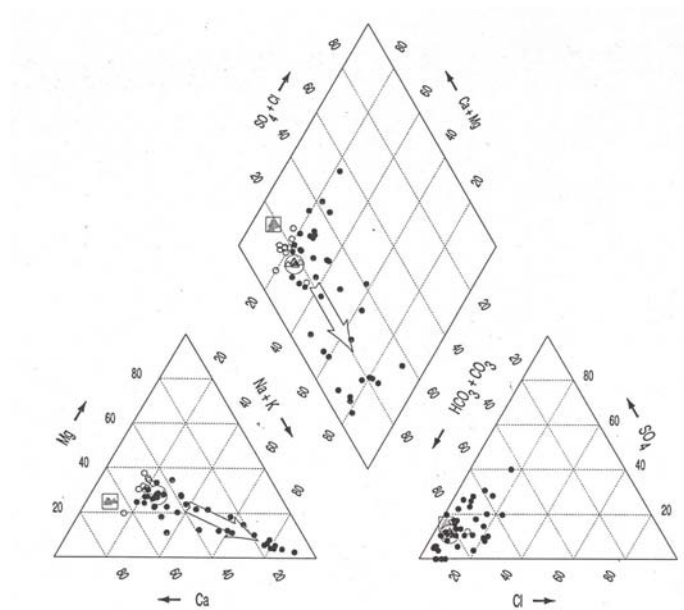
Figure 4. Tri-linear diagram that (a) compares chemical composition between Selah (red symbol) and Mabton (white symbol) interbeds and (b) Hanford site-Pasco Basin Upper-Saddle Mountains Basalt / Ellensburg Formation groundwaters (from Spane, 2004)
