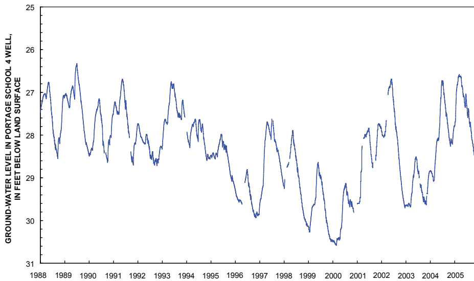
Figure 11. Depth below land surface of water in Portage School 4 well, Kalamazoo County, January 1988 through December 2005.
