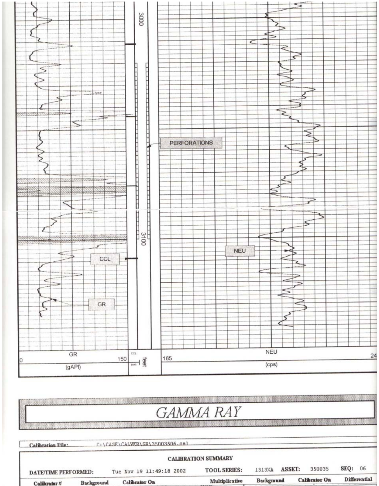
Figure 39: Pre-Sonication Gamma Ray/Neutron Log
