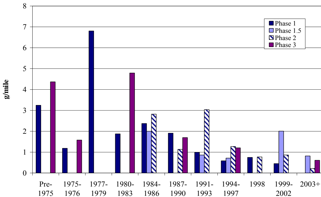
Figure 58: Variation of HHTDT oxides of NO x by vehicle model year and by phase of the program for the UDDS (56,000 lbs.).
