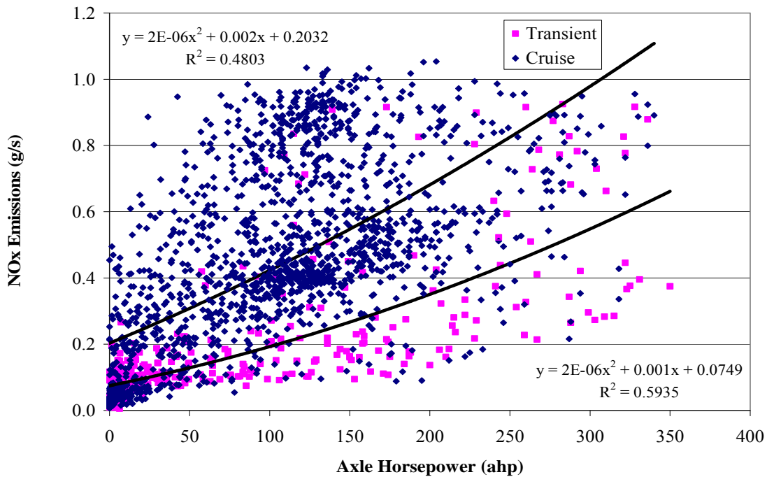
Figure 128: NO x emissions versus power for E55CRC-10 after reflashing. The mass rate of NO x emissions was reduced in many parts of the Cruise mode (compared to Figure 122). The highest mass rate emissions were also slightly lower than before the reflash.
