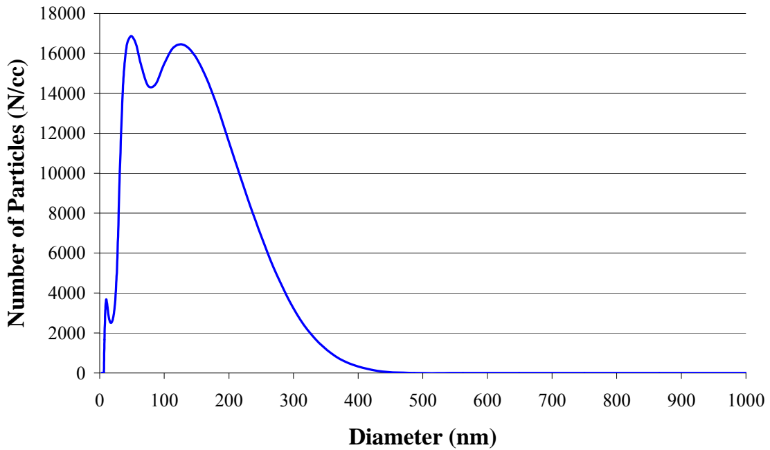
Figure 74: DMS500 size distribution of particles during acceleration (t = 530 s) of the UDDS for E55CRC-39 tested at 56,000 lbs.
