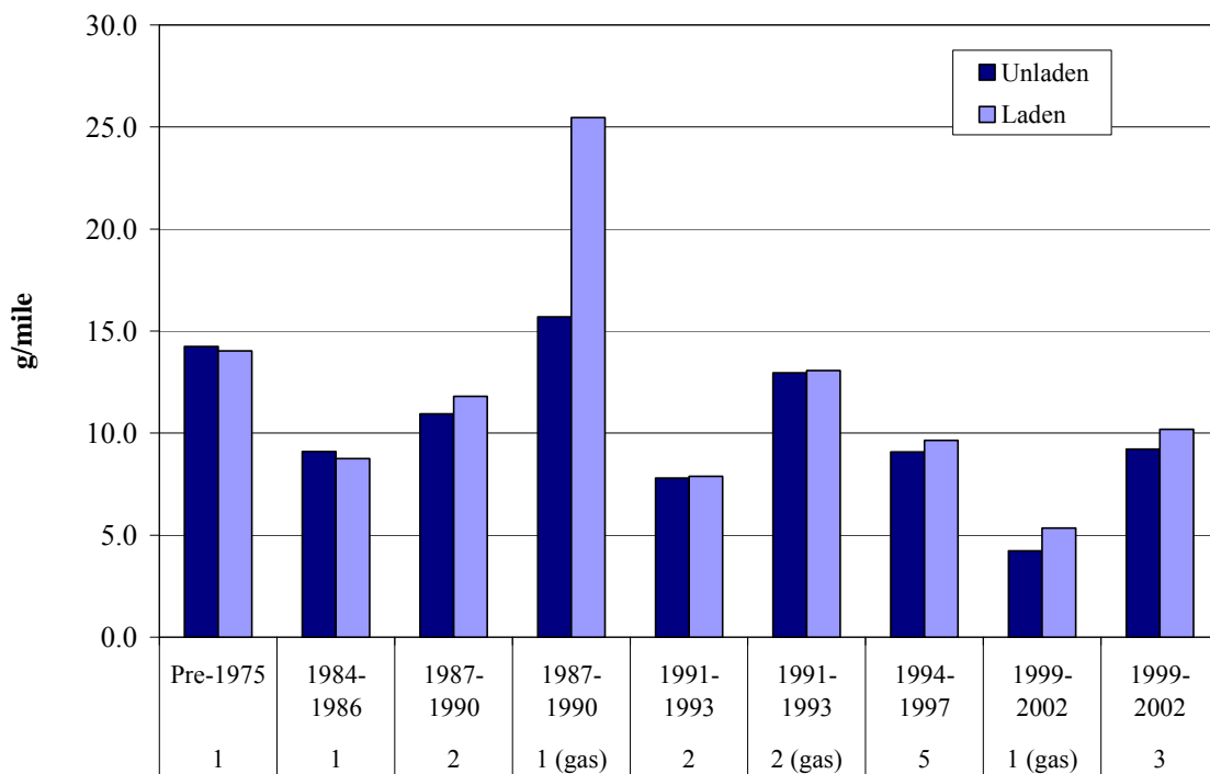
Figure 35: NO x emissions for the MHDT Cruise mode (both laden and unladen).
