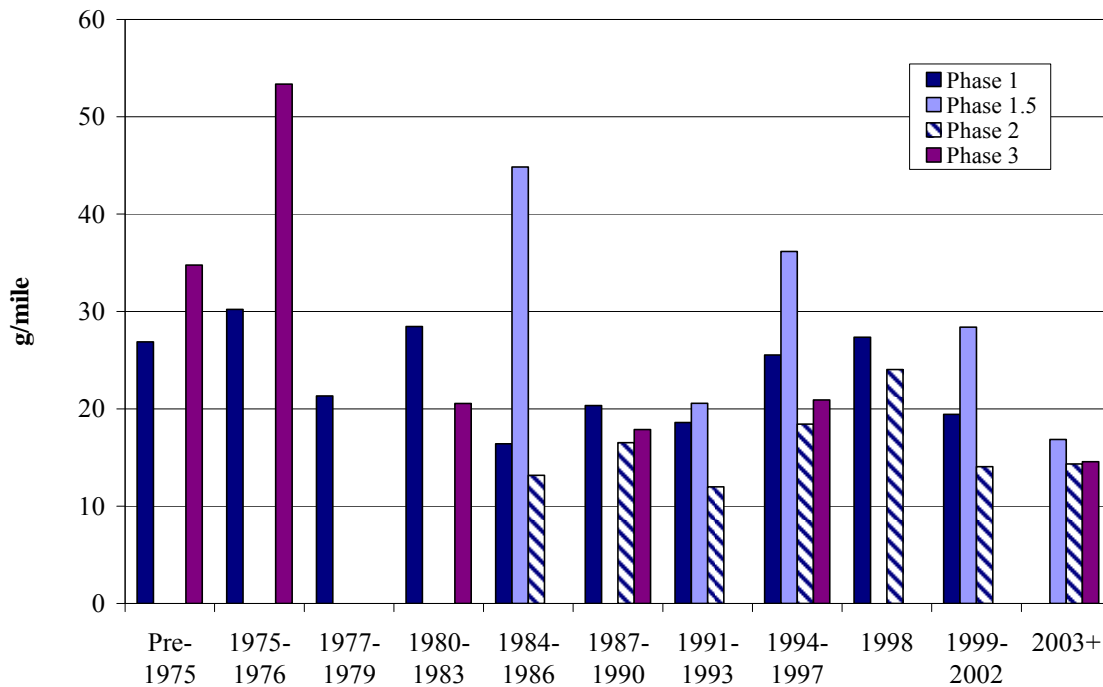
Figure 58: Variation of HHTDT oxides of NO x by vehicle model year and by phase of the program for the UDDS (56,000 lbs.).
