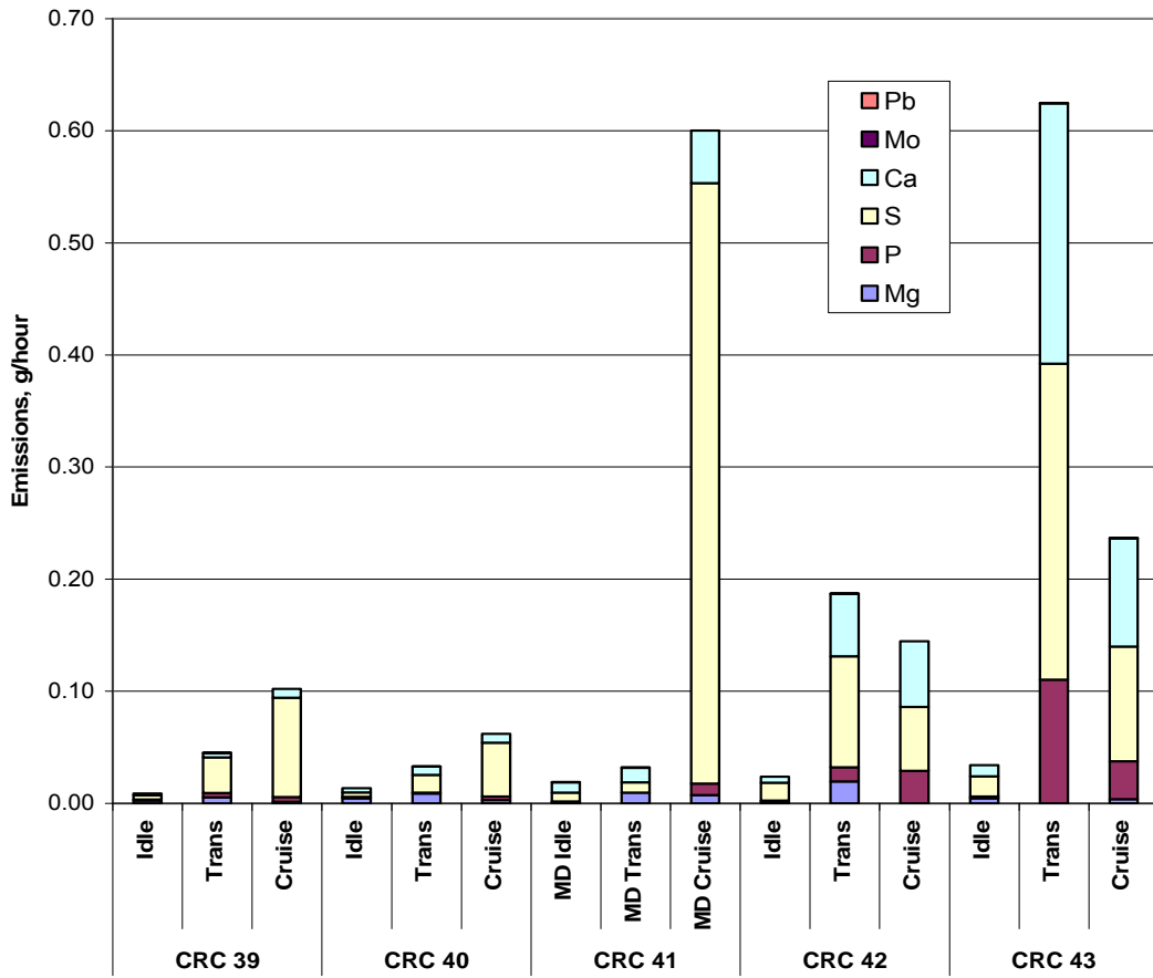
Figure 19: Lubrication Oil Emissions
