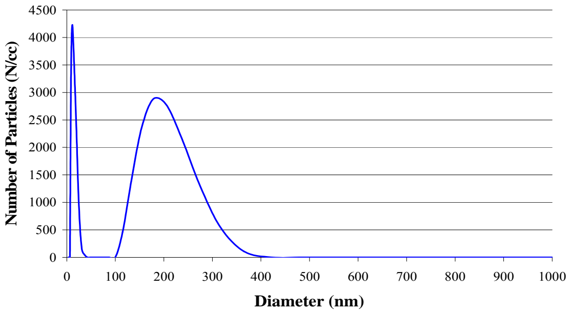
Figure 75: DMS500 size distribution of particles during deceleration (t = 770 s) of the UDDS for E55CRC-39 tested at 56,000 lbs.
