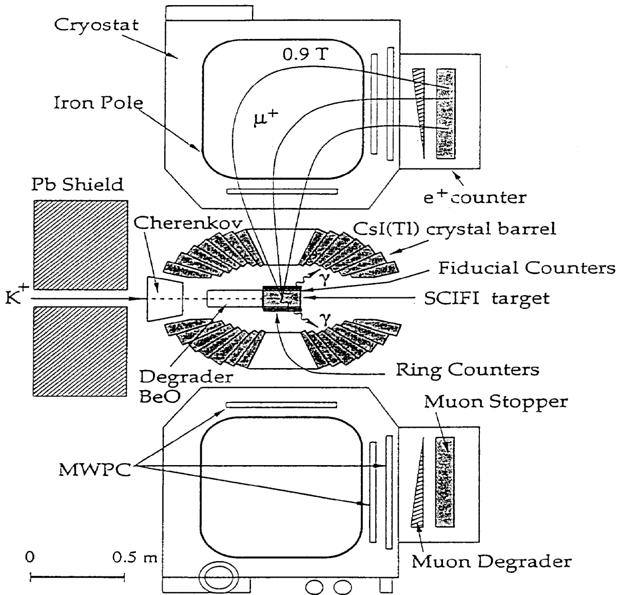
Cross-Section View of the E936 Detector Set Up
