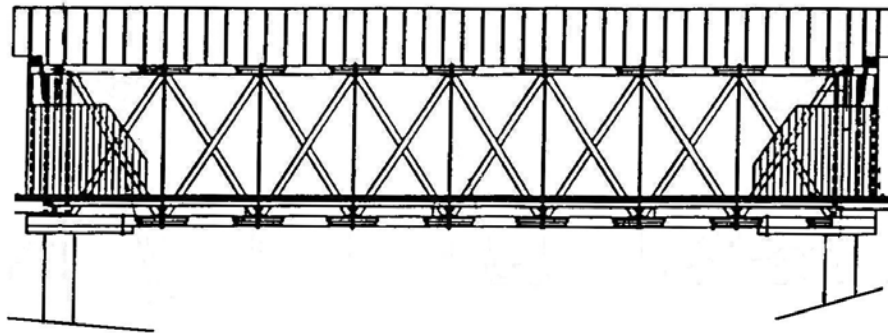
Figure 7 Side view of Hammond Bridge truss system (exterior siding not shown), floor, and rafters. (Adapted from Shuck-Britson Inc. rehabilitation plans dated January 2003)
