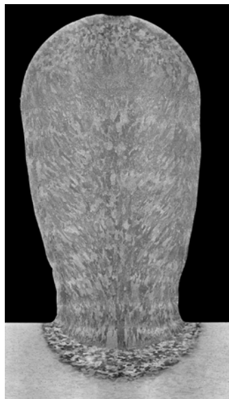
Figure 5. Microstructure for preheat pass plus 10 layers (20 kV accelerating voltage shown).
