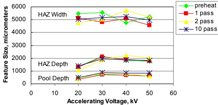
Figure 6. Influence of accelerating voltage on the width and depth of heat affected zone, and depth of molten pool into the baseplate for several different height EBF 3 deposits.
