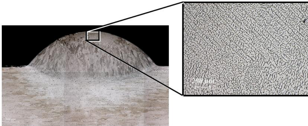
Figure 3. Microstructure of preheat pass plus single layer deposit for 20 kV accelerating voltage.
