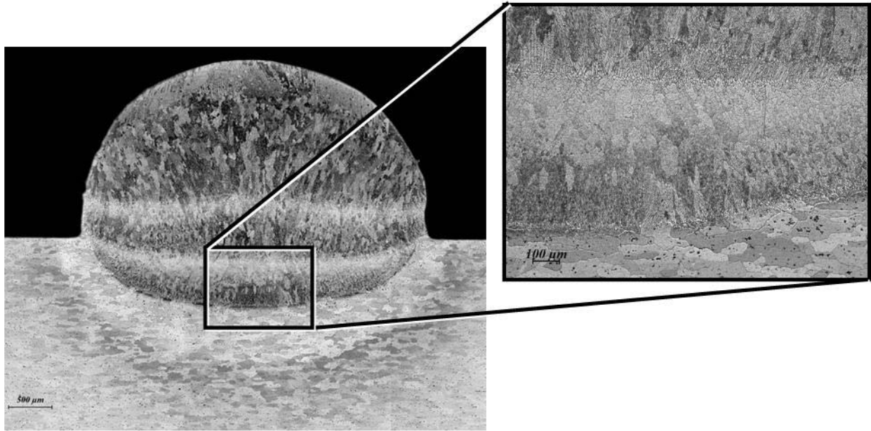
Figure 4. Representative microstructure for preheat pass plus two layers (40 kV accelerating voltage shown).
