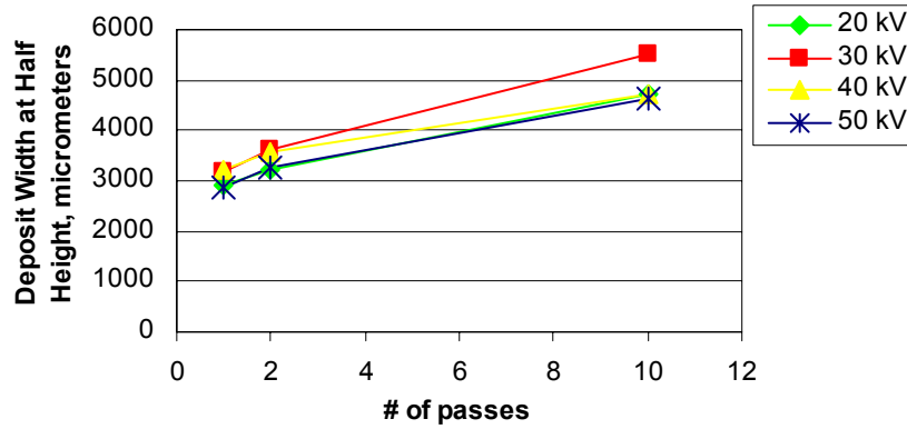
Figure 7. Widths of EBF 3 deposits, measured at half the height above the baseplate, increase with increasing deposit heights.
