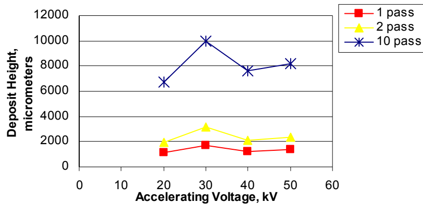
Figure 8. Heights of EBF 3 deposits are not affected by the beam accelerating voltage.
