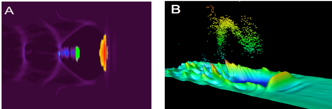
Figure 1. Schematic of an LWFA, from a VORPAL 3D simulation on 4096 processors of a centimeter-scale 0.7 GeV stage (A): the radiation pressure of a laser pulse (red) displaces plasma electrons creating a space charge wave (purple-blue) which accelerates particles, creating a compact bunch (green). Simulations resolve phase space and internal dynamics to optimize WFAs, showing for instance (B) particles in px - x - y space above plasma density in a 100 MeV self-trapped stage (VORPAL 3D).
