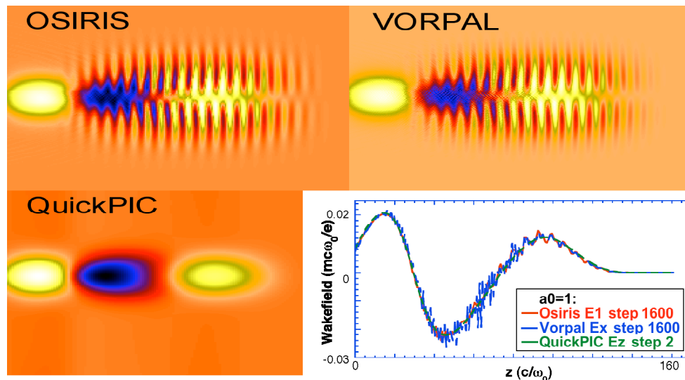
Figure 2. 3D simulation results from OSIRIS, VORPAL, and QuickPIC for an LWFA benchmark problem with a_0=1 show good agreement. The normalized accelerating wakefield is shown as a 2D slice (upper and left), and also overlapping lineouts down the center (lower right).
