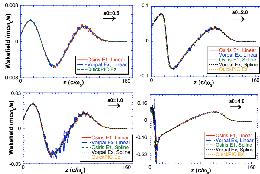
Figure 3. Overlapping lineouts down the center of the simulation domain show good agreement between 3D OSIRIS, VORPAL and QuickPIC simulations of the LWFA benchmark problem for a_0=0.5, 1, 2, and 4 , including the use of second-order spline-based particle shapes.
