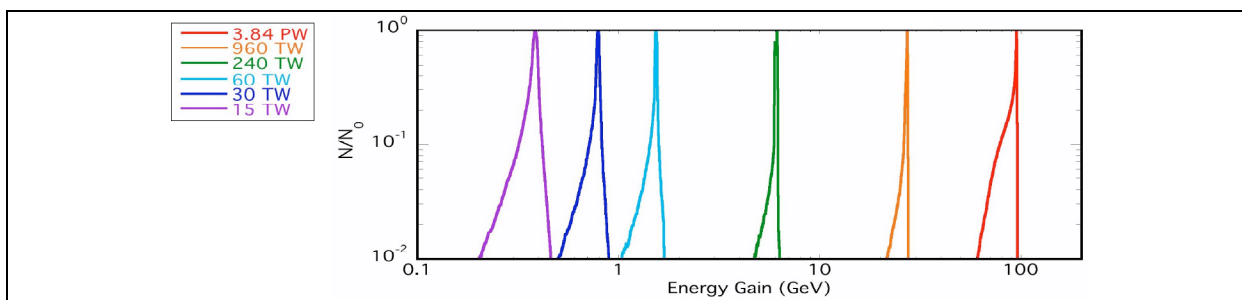
Figure 5. Final electron spectra for a series of LWFA simulations in the nonlinear blowout regime for P/P_c=1 . In each case a trailing bunch of electrons was injected. The energy gain is shown, where each color corresponds to a different laser power. Energy gain agreed with scalings (QuickPIC).
