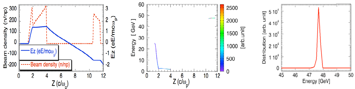
Figure 6. A witness beam with initial energy of 25 GeV and 1.7 \times 10^{10} electrons gains \sim 25 GeV energy with 0.46% energy spread in a PWFA simulation. The plasma is preionized. Left: the density profile of the drive and witness beam and the longitudinal wake they generated. Middle: Phase space plot of the drive and witness beam, showing energy doubling of the witness beam and depletion of the energy of the drive beam. Right: Energy distribution of the accelerated witness beam (QuickPIC).
