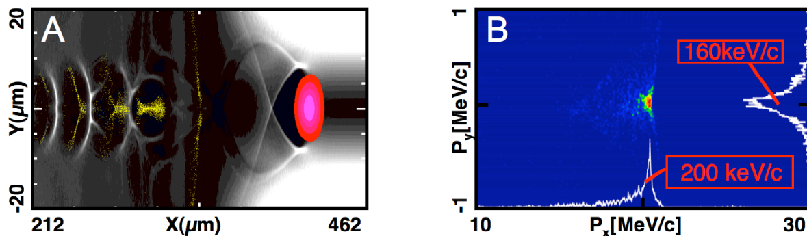
Figure 4. VORPAL simulations merging density gradient injection to an accelerating channel (A) show the laser (red), plasma wake density (grey) and accelerating particles (yellow). Acceleration in the channel (B) produces 20 MeV bunches and preserves the bunch's 0.2 MeV/c momentum spread.
