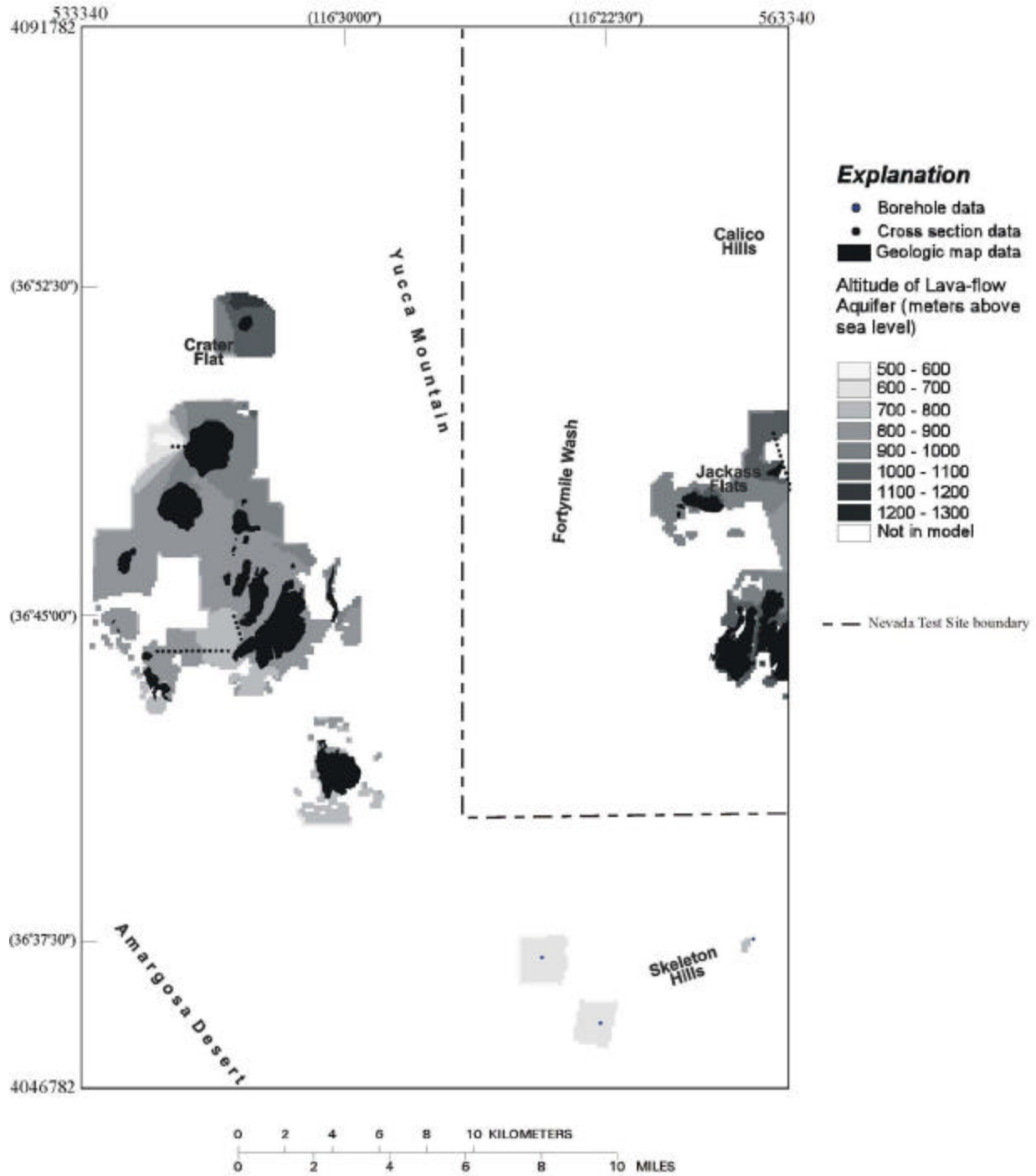
Figure 6-5. Map Showing Distribution of Lava-Flow Aquifer and Data Distribution used to Construct Surface (Unit distribution is before clipping by potentiometric surface) (DTN: GS000508312332.002)
