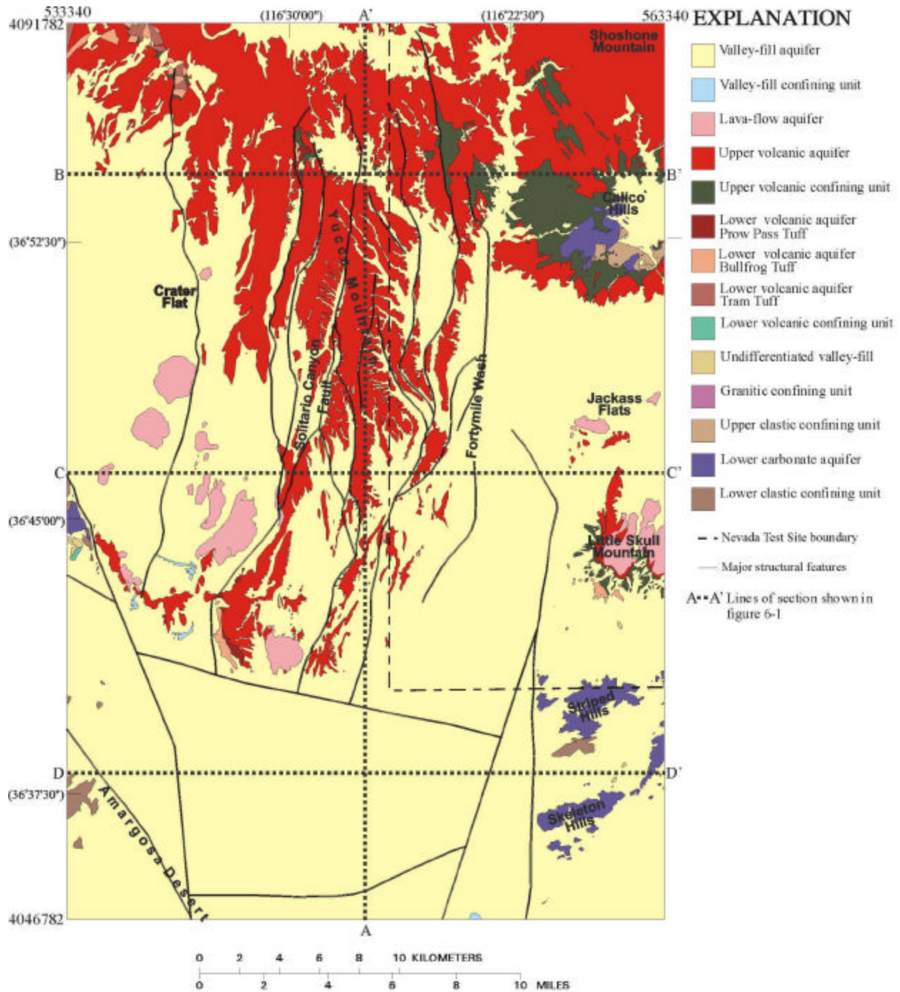
Figure 4-2. Generalized Surface Outcrop Map of Hydrogeologic Units with Major Structural Features and Lines of Section Specific to the Site Model Area (DTN: GS991208314221.001)
