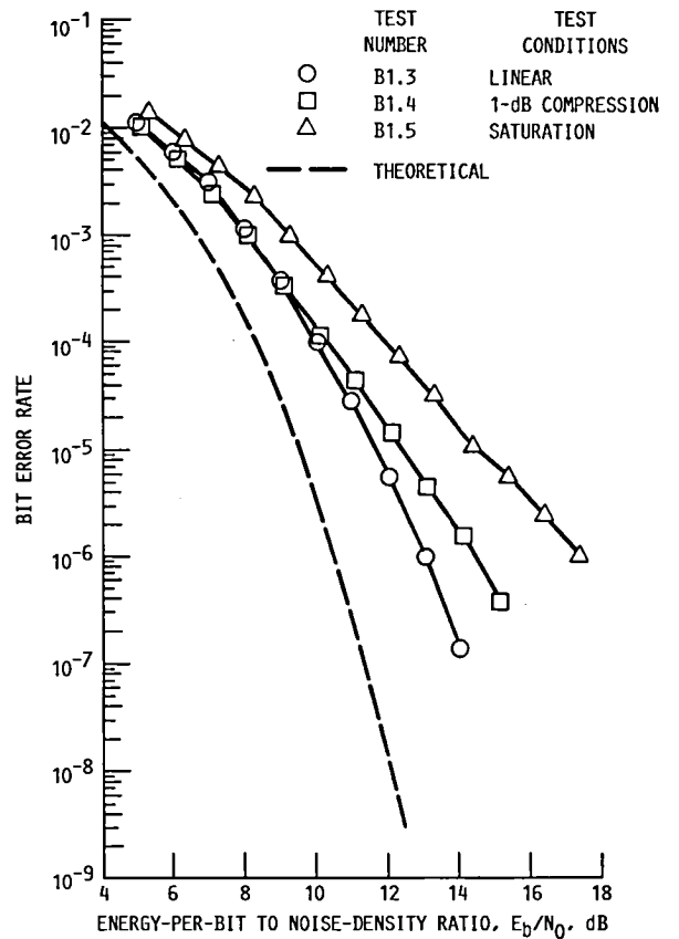
FIGURE 12. - LINK BIT-ERROR-RATE PERFORMANCE FOR TRAVELING WAVE TUBE IN MEDIUM MODE.
