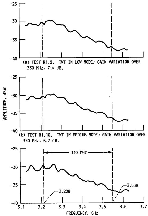
FIGURE 10. - FREQUENCY RESPONSE TESTS FOR TRAVELING WAVE TUBE (TWT) AT BASELINE.
