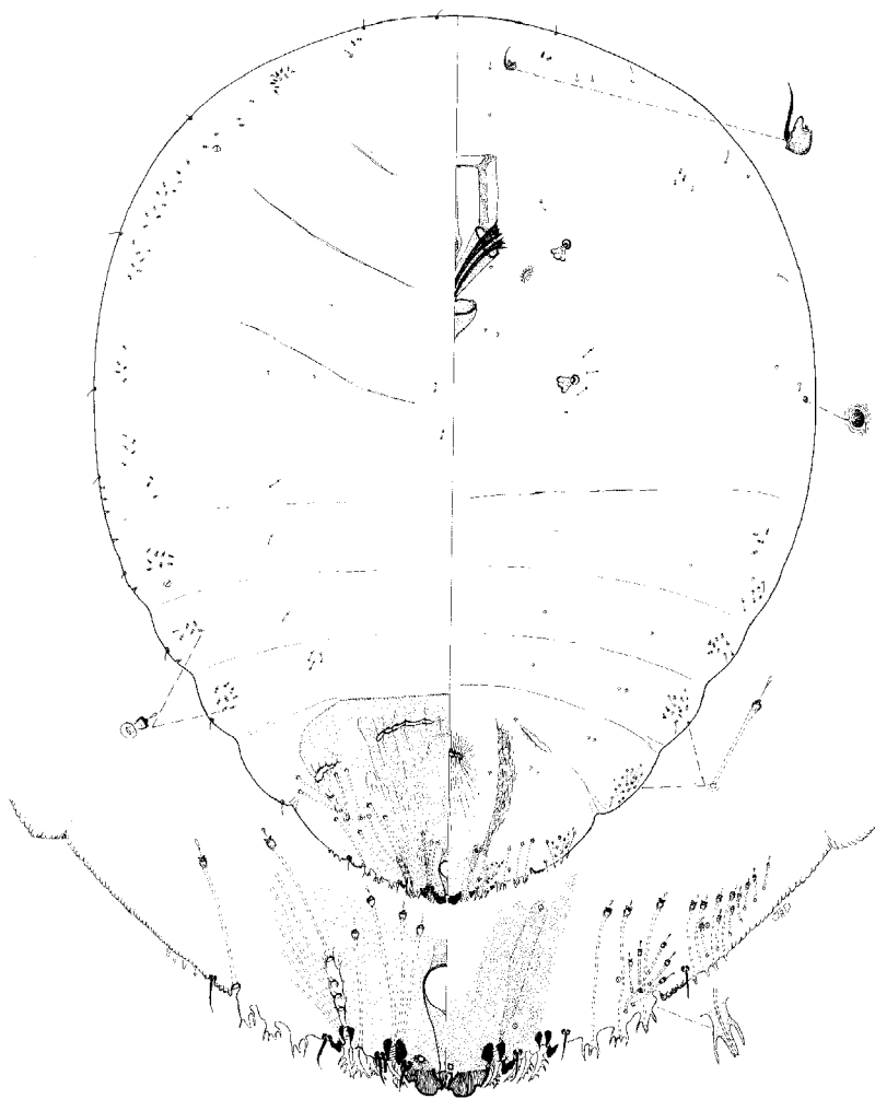
Fig. 1. Adult female holotype Hemiberlesia neodiffinis . Simpson, Illinois, August 7, 1969, on Liriodendron tulipifera . J. E. Appleby.
