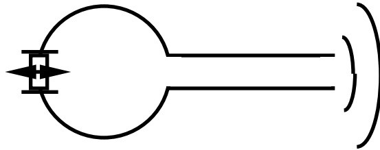
Figure I.2: Driven, radiating Helmholtz resonator.
