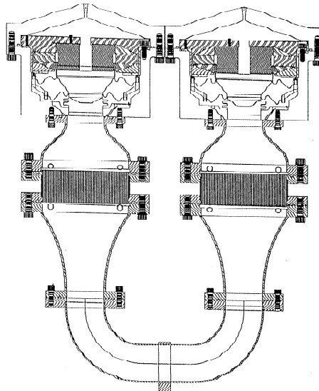
Figure I.5: Thermoacoustic refrigerator (TALSR style)
