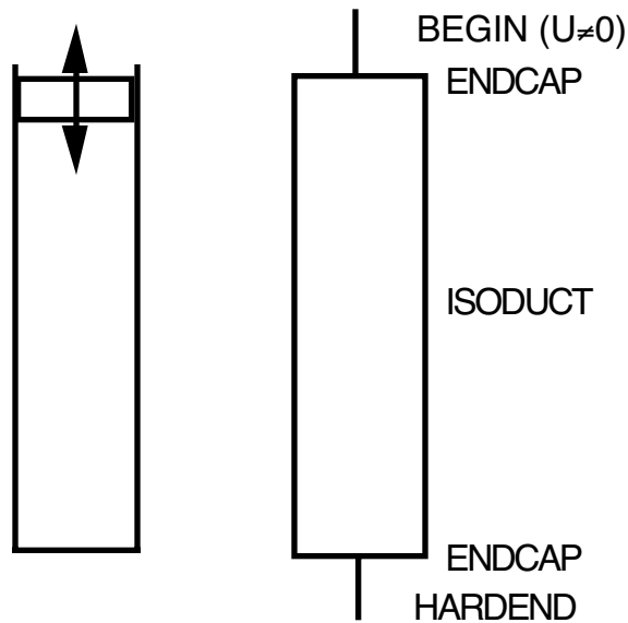
Figure II.1: A plane-wave resonator; conventional and DELTAE representation.
