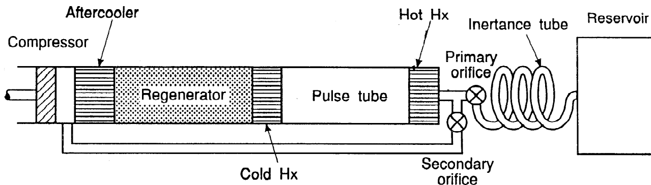
Figure I.9: Double-inlet pulse-tube refrigerator.
