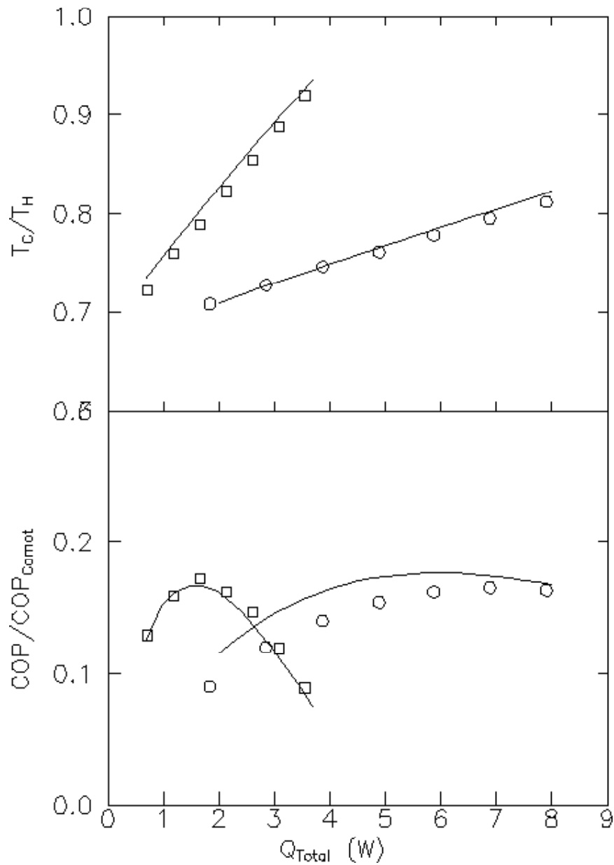
Figure III.4: Hofler refrigerator results. Lines are DELTAE results; points are from experimental data presented in Hofler's thesis. Squares, p_1 = 0.015p_m . Circles, p_1 = 0.03p_m .
