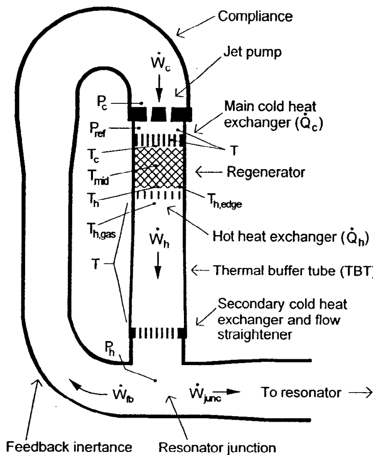
Figure I.8: Thermoacoustic Stirling hybrid engine.
