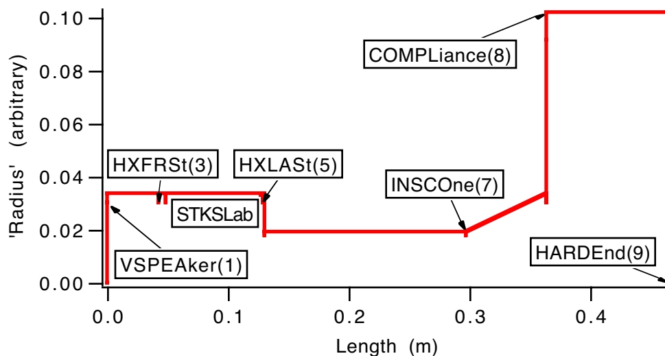
Figure V.3: Geometry of Hoffer refrigerator example.
