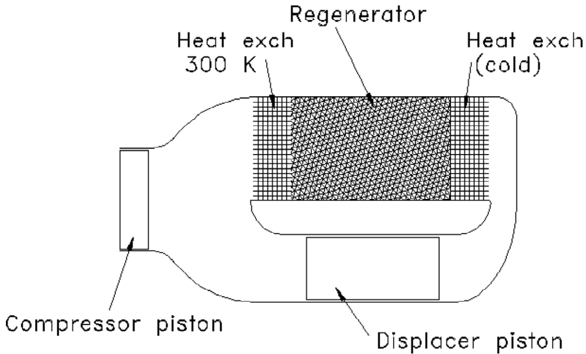
Figure V.2: "Gamma"-style Stirling machine.
