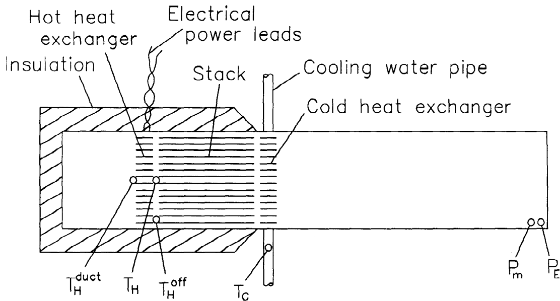
Figure III.1: 5-inch engine.
