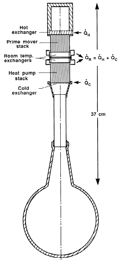
Figure I.7: Beer cooler.
