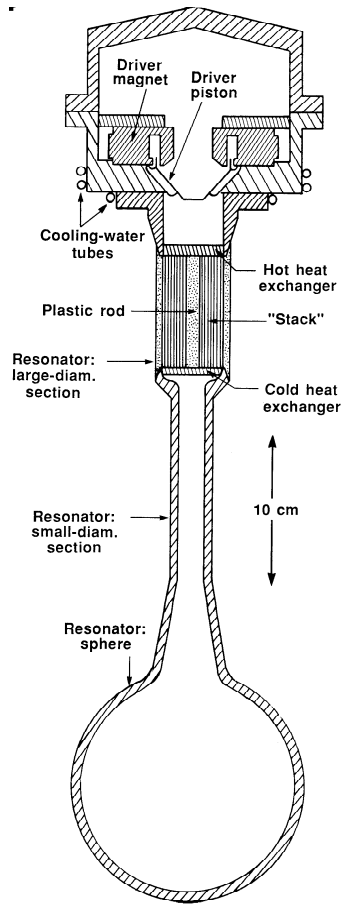
Figure I.4: Thermoacoustic refrigerator (Hoffer style).
