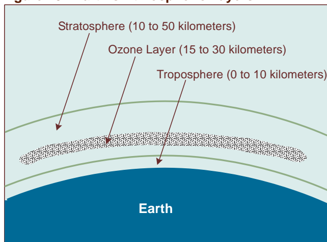
Figure 13. Earth's Atmospheric Layers
