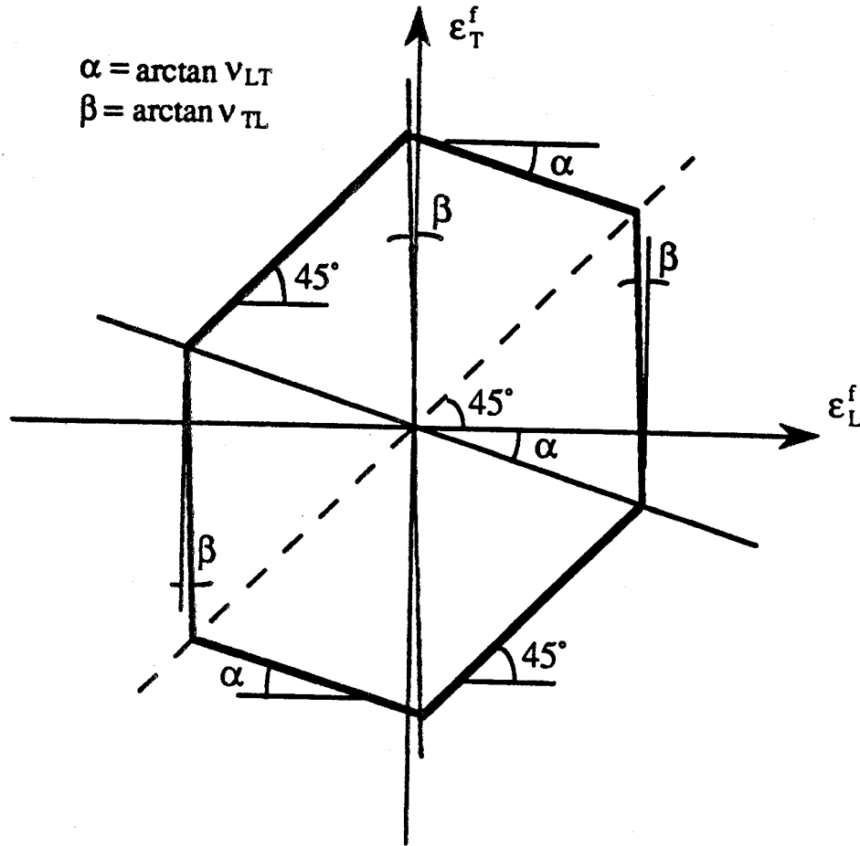
FIGURE 24. FAILURE STRAIN ENVELOPE PROPOSED BY HART-SMITH FOR FIBERS
