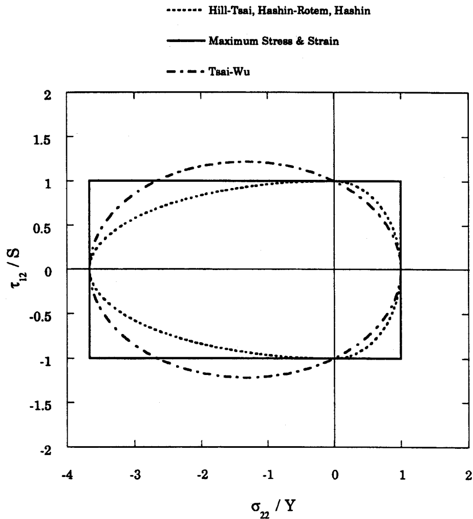
FIGURE 4. COMPARISON OF LAMINA FAILURE CRITERIA UNDER \sigma_{22} - \tau_{12} BIAXIAL STRESS
