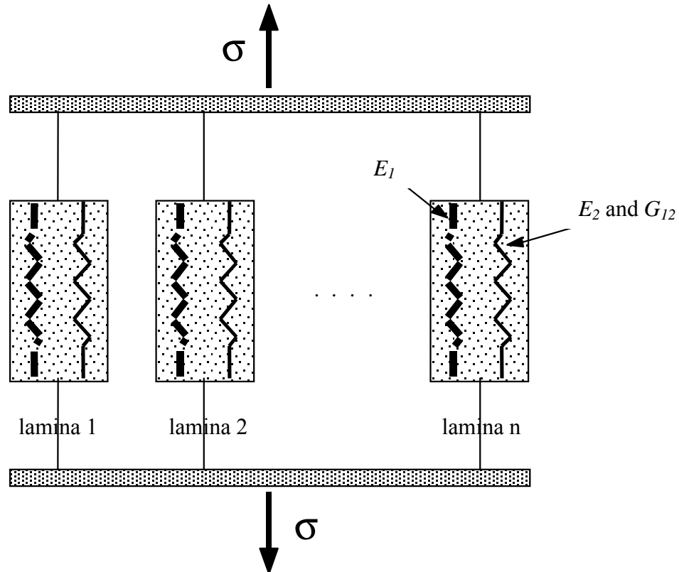
FIGURE 21. SCHEMATIC OF THE PARALLEL STIFFNESS MODEL
