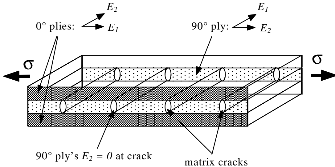
FIGURE 22. SCHEMATIC OF LAMINATE WITH MATRIX CRACKS
