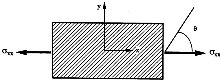
FIGURE 5. OFF-AXIS LOADING OF A LAMINA
