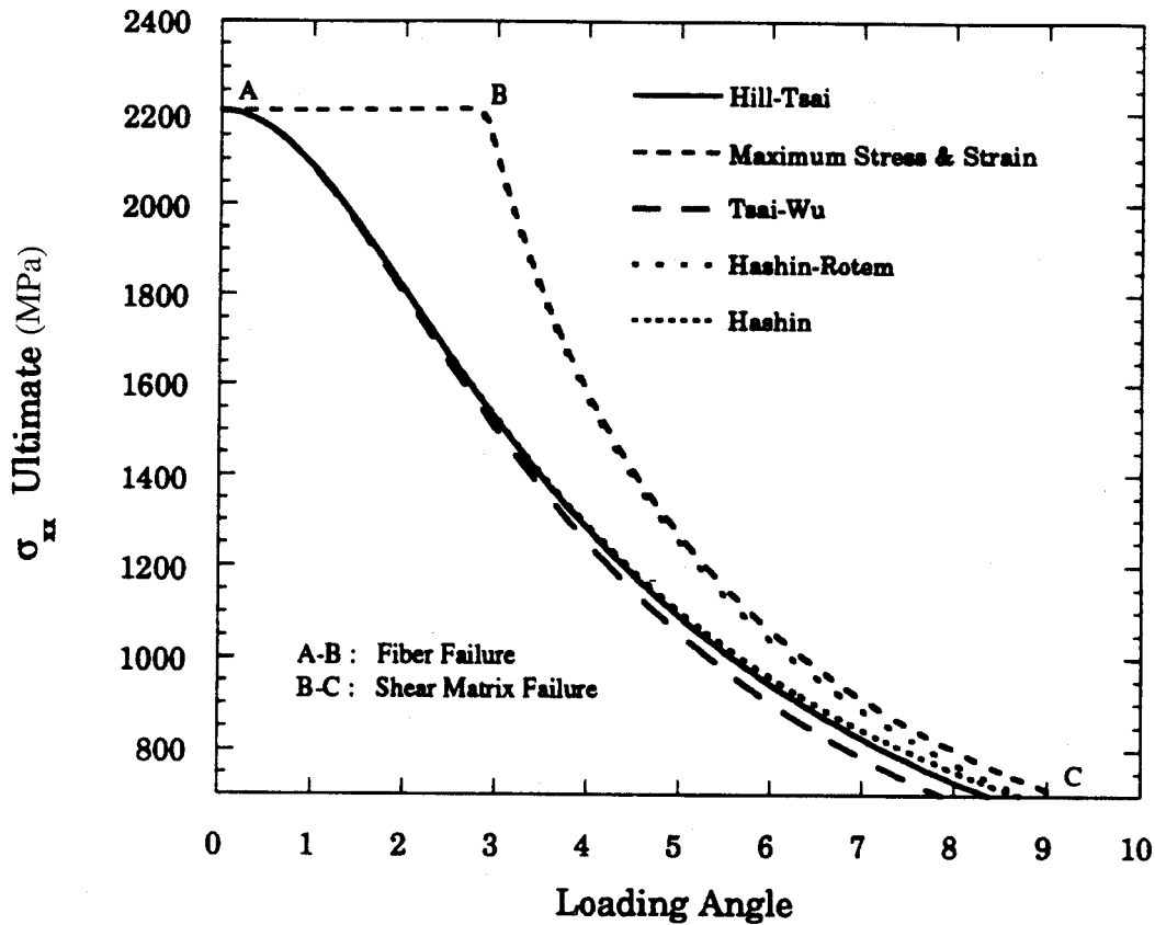
FIGURE 7. DETAILED COMPARISON OF LAMINA FAILURE CRITERIA FOR OFF-AXIS LOADING
