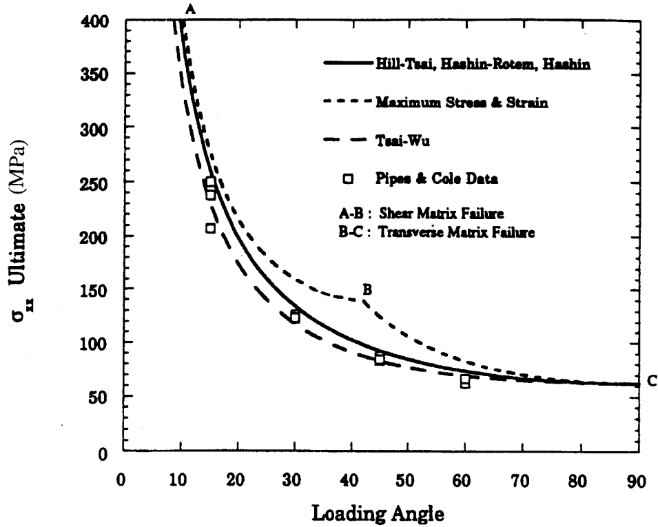
FIGURE 10. COMPARISON OF LAMINA FAILURE CRITERIA TO OFF-AXIS DATA
