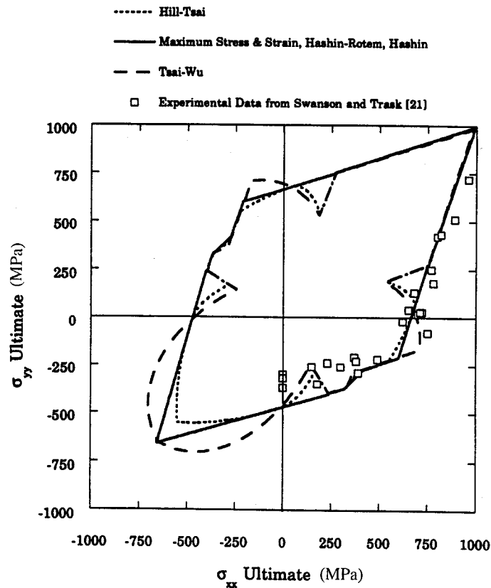
FIGURE 29. COMPARISON OF ULTIMATE STRESS ENVELOPES WITH EXPERIMENTAL DATA FOR A [0/\pm 45/90]_s LAMINATE UNDER BIAXIAL LOADS
