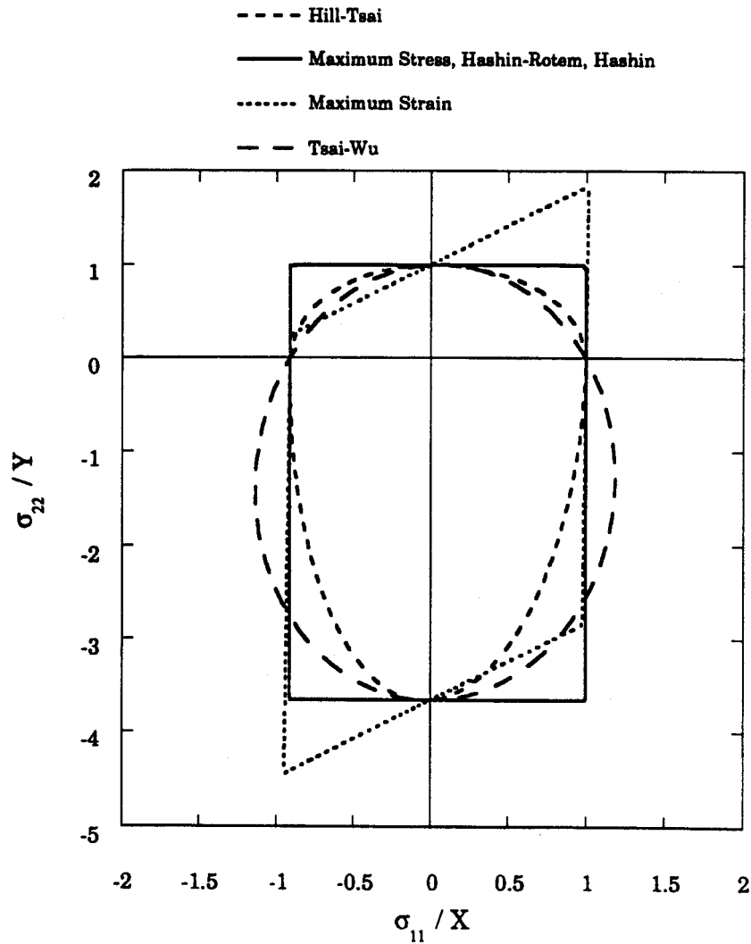
FIGURE 2. COMPARISON OF LAMINA FAILURE CRITERIA UNDER \sigma_{11} - \sigma_{22} BIAXIAL STRESS
