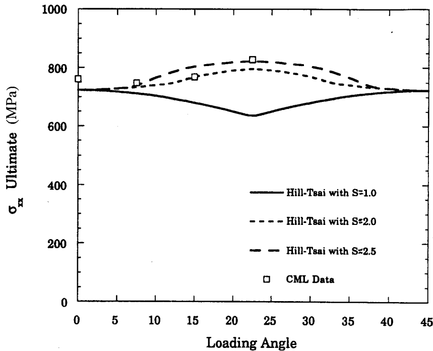
FIGURE 42. COMPARISON OF ULTIMATE STRENGTHS FOR A [0/A/+45/A/-45/A/90]_s WITH DIFFERENT LAMINA SHEAR STRENGTHS USING HILL-TSAI CRITERION
