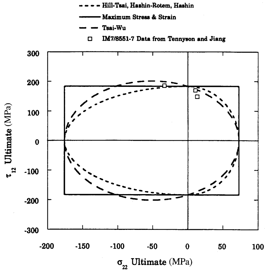
FIGURE 14. COMPARISON OF LAMINA FAILURE CRITERIA TO \sigma_{22} - \sigma_{12} DATA FROM TENNYSON AND JIANG
