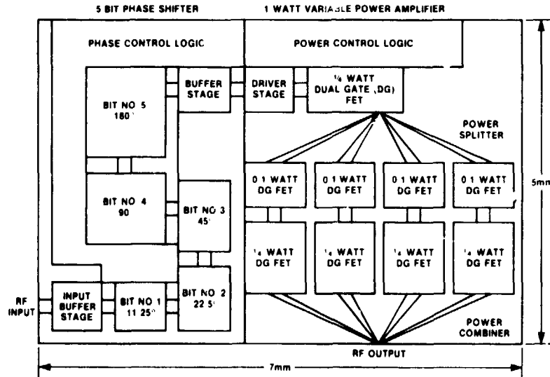
Figure 10. - 20 GHz GaAs monolithic transmit module.
