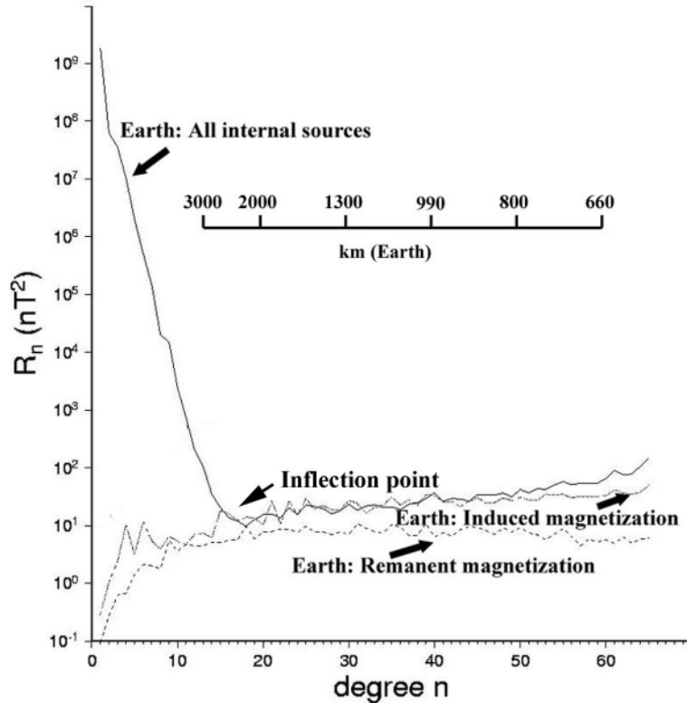
Figure 8. Comparison of the Lowes-Mauersberger ( R_n ) spectra at the surface of the Earth for a variety of internal fields. The inflection point in the terrestrial power spectra represents the sharp transition from core processes at low n to lithospheric processes at higher n . R_n is the mean square amplitude of the magnetic field over a sphere produced by harmonics of degree n . The spectrum of all internal sources comes from Sabaka et al. (2004), the induced spectrum is derived from Fox Maule et al. (2005), and the remanent magnetization spectrum (of the oceans, and hence a minimum value) was derived from Dymnt and Arkani-Hamed (1998).
