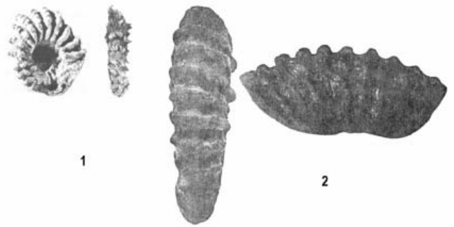
Figure 13. Ammonites fossils from turbidite sandstones of the Marin Headlands Terrane.
