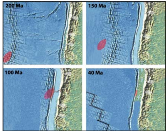
Figure 6. Transport history of the Marin Headlands Terrane across the Pacific basin. Panels show approximate geographic position of terrane, shown as red area, at 200, 150, 100, and 40 million years ago (modified from Murchey and Jones, 1984).
