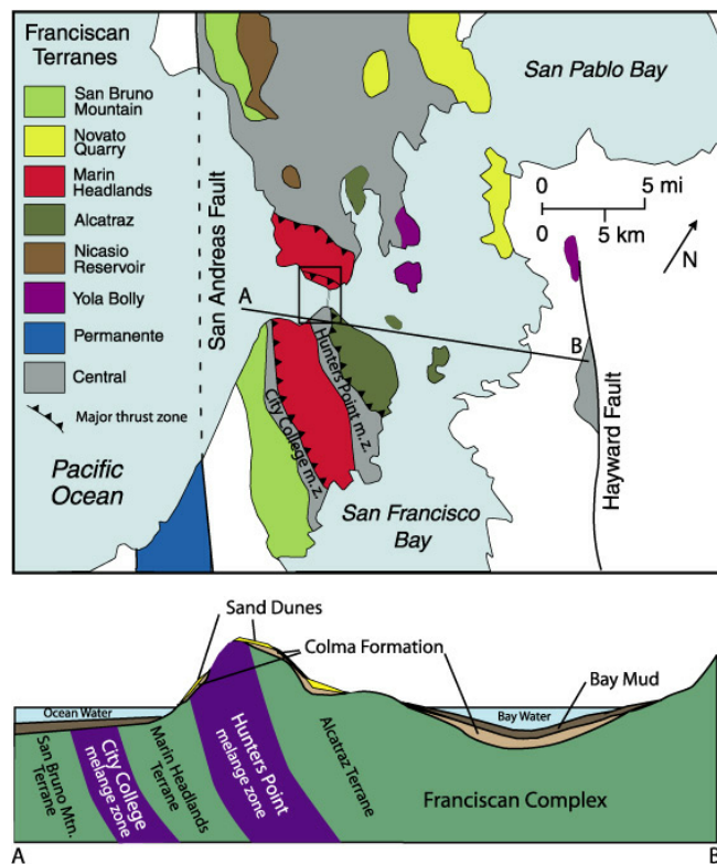
Figure 2. Top part of figure shows terranes of the Franciscan Complex in the San Francisco Bay Area and dip direction of major thrust faults referred to in text. Cross section A-B for lower part of figure also is indicated (modified from Blake et al., 1984). Bottom part of figure is a schematic cross-section through northern San Francisco Peninsula across bay to Oakland (not to scale).
