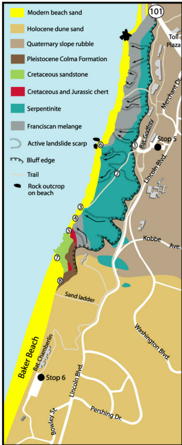
Figure 5. Geologic map of coastal bluffs in the Presidio showing major geologic units, location of field trip stops, and locations at stops referred to in text (modified from Wahrhaftig, 1984b; Schlocker, 1974). Arrows indicate the direction of landslide movement.
