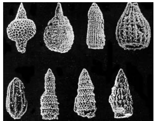
Figure 10. Scanning electron micrographs of silica tests (shells) of Radiolaria removed from the Marin Headlands chert by using hydrofluoric acid (from Murchey, 1984).
