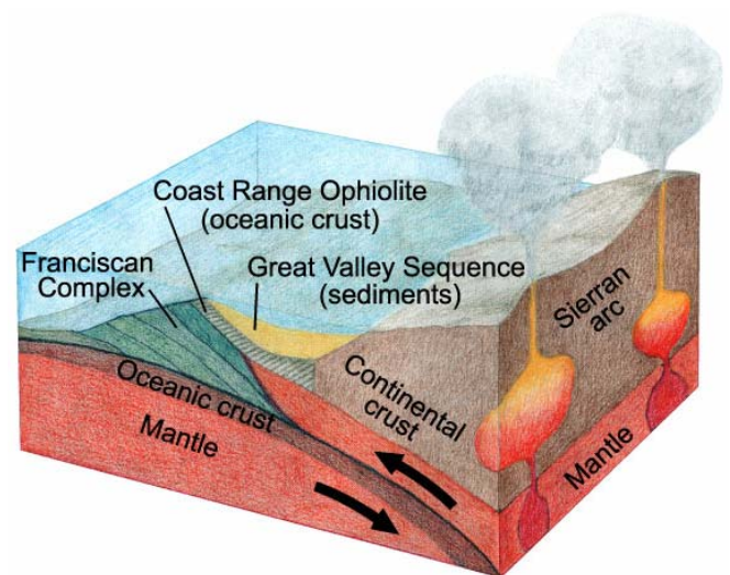
Figure 3. Cartoon of the subduction zone present on the West Coast 100 million years ago showing position of the Franciscan accretionary complex.
