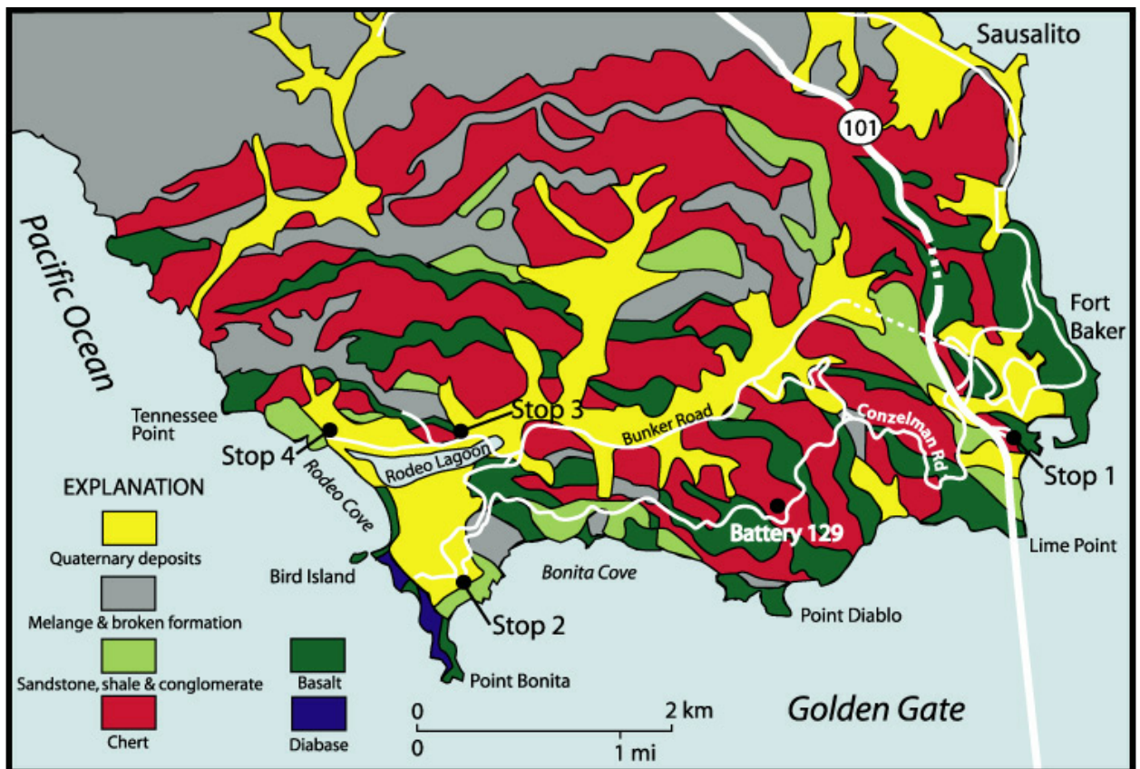
Figure 4. Geologic map of the Marin Headlands showing major geologic units, location of field trip stops, and other places referred to in text (modified from Wahrhaftig and Murchey, 1987).
