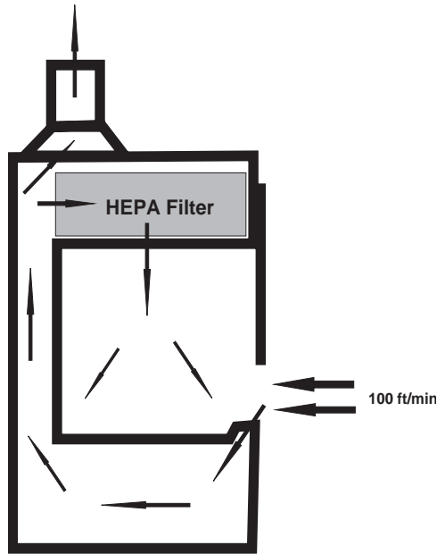
BSC Airflow
