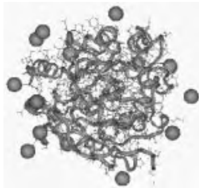
This image is from a simulation of a halo-alkane dehalogenase enzyme after 100 picoseconds. The simulation was performed by molecular dynamics software that uses global arrays, part of DOE's ACTS toolkit.
