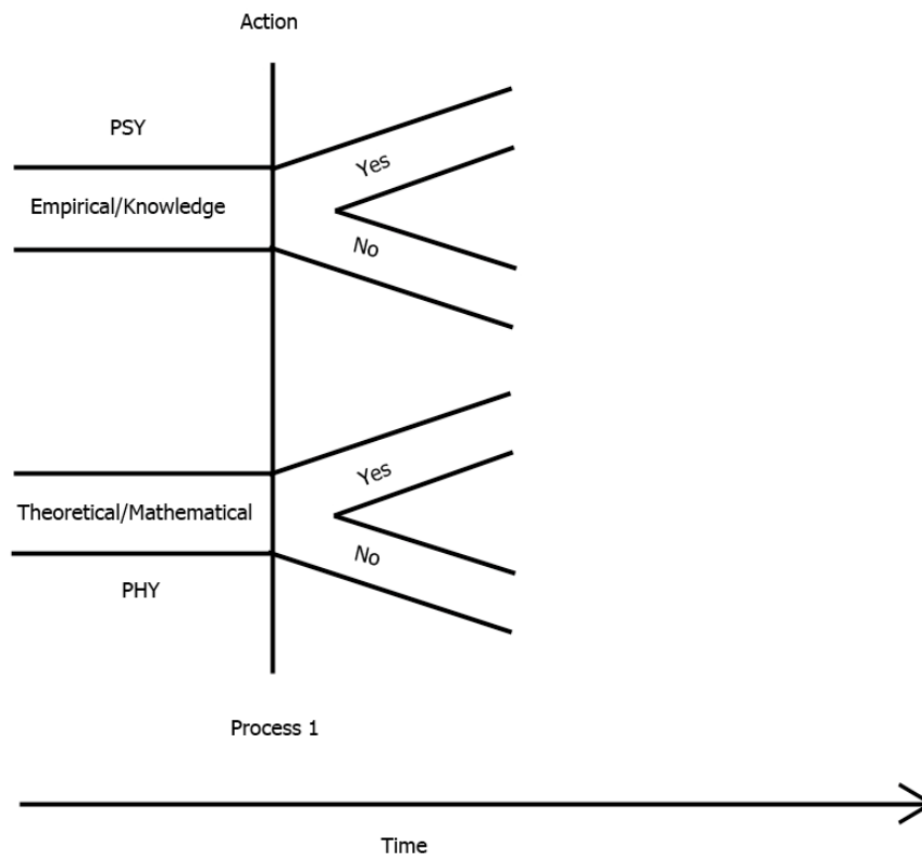
Figure 3. The action associated with Process 1. Each empirical finding is associated with a process 1 quantum reduction event that has both an experiential part that
