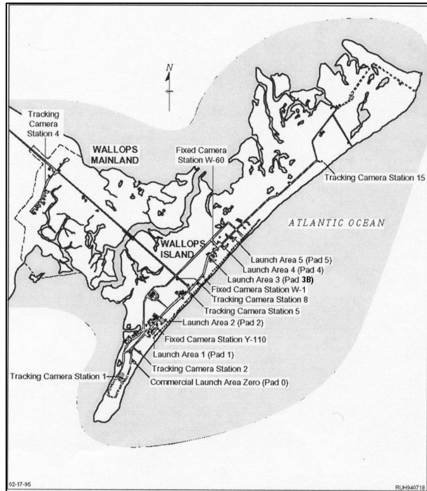
Figure 3-21. Optical Tracking Stations at Wallops Island and Mainland
