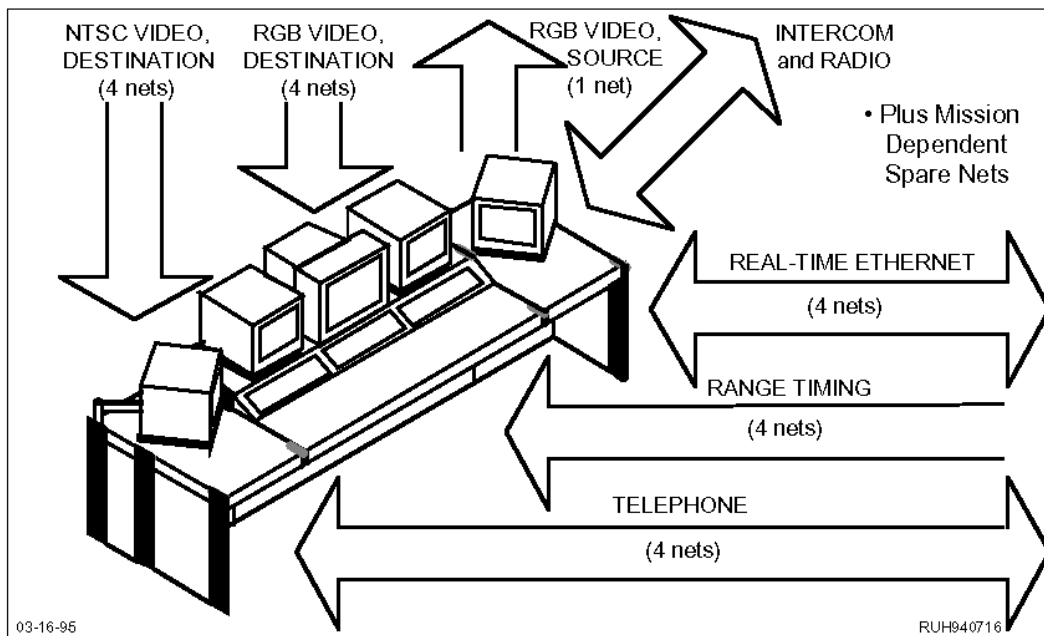
Figure 3-18. Mission Controller Station Data Interfaces
