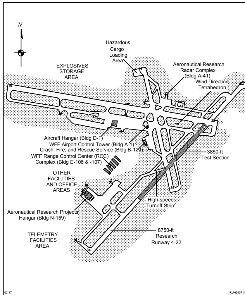
Figure 3-14. WFF Research Airport with Associated Facilities
