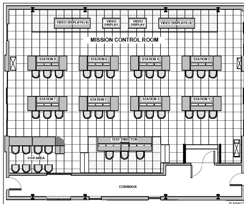
Figure 3-16. Layout of RCC Mission Control Room
