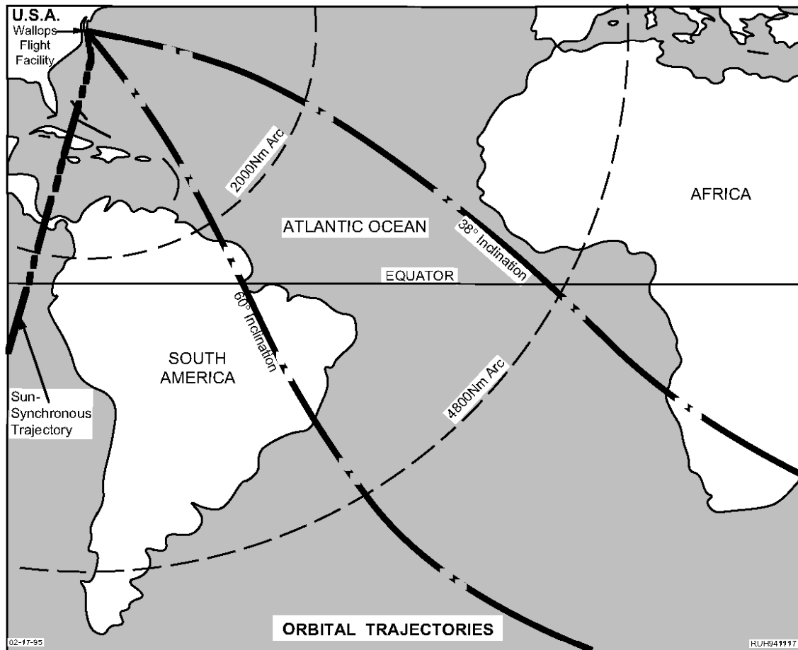
Figure 3-6. Orbital Trajectories
