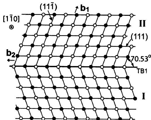
FIG. 1. Illustration of a regular twin (step 1). The open and filled circles represent atoms from two adjacent (1\bar{1}0) planes, respectively.
