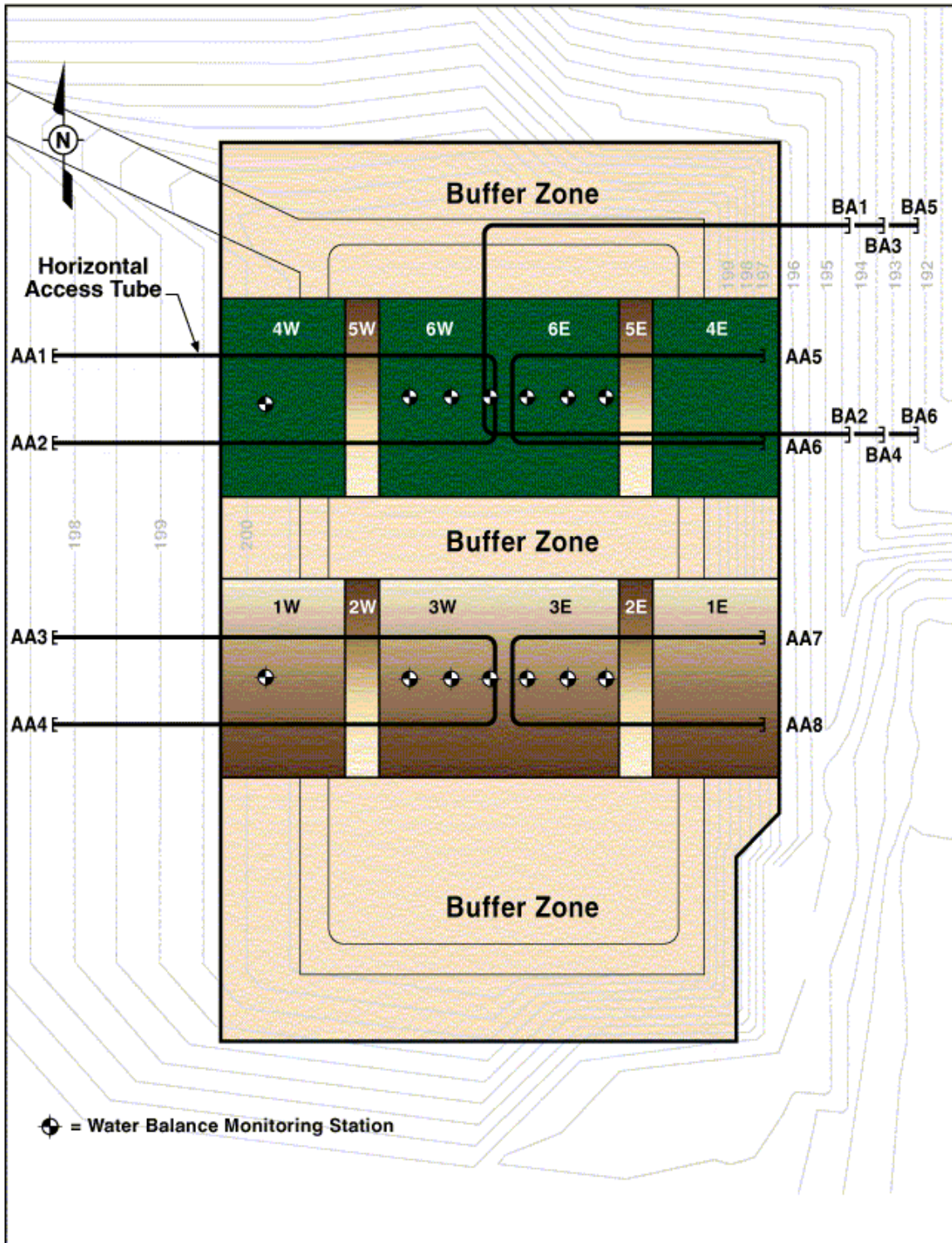
Figure 2.7. Plan View of the Barrier Showing the Layout of the 12 Surface Soil Plots (1W to 6W and 1E to 6E) and Horizontal Neutron Access Tubes (AA-Above Asphalt; BA-Below Asphalt)
