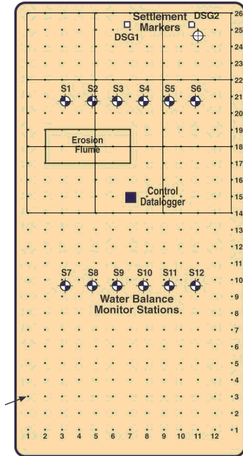
Figure 3.1. Schematic Plan View of the Barrier's Surface Showing Monitoring Stations, the Runoff Plot, the 3 × 3 M Grid, and the Nine 12 × 12 M Plots to Be Used for Comparing Fuel Loads on Fire Intensity.
