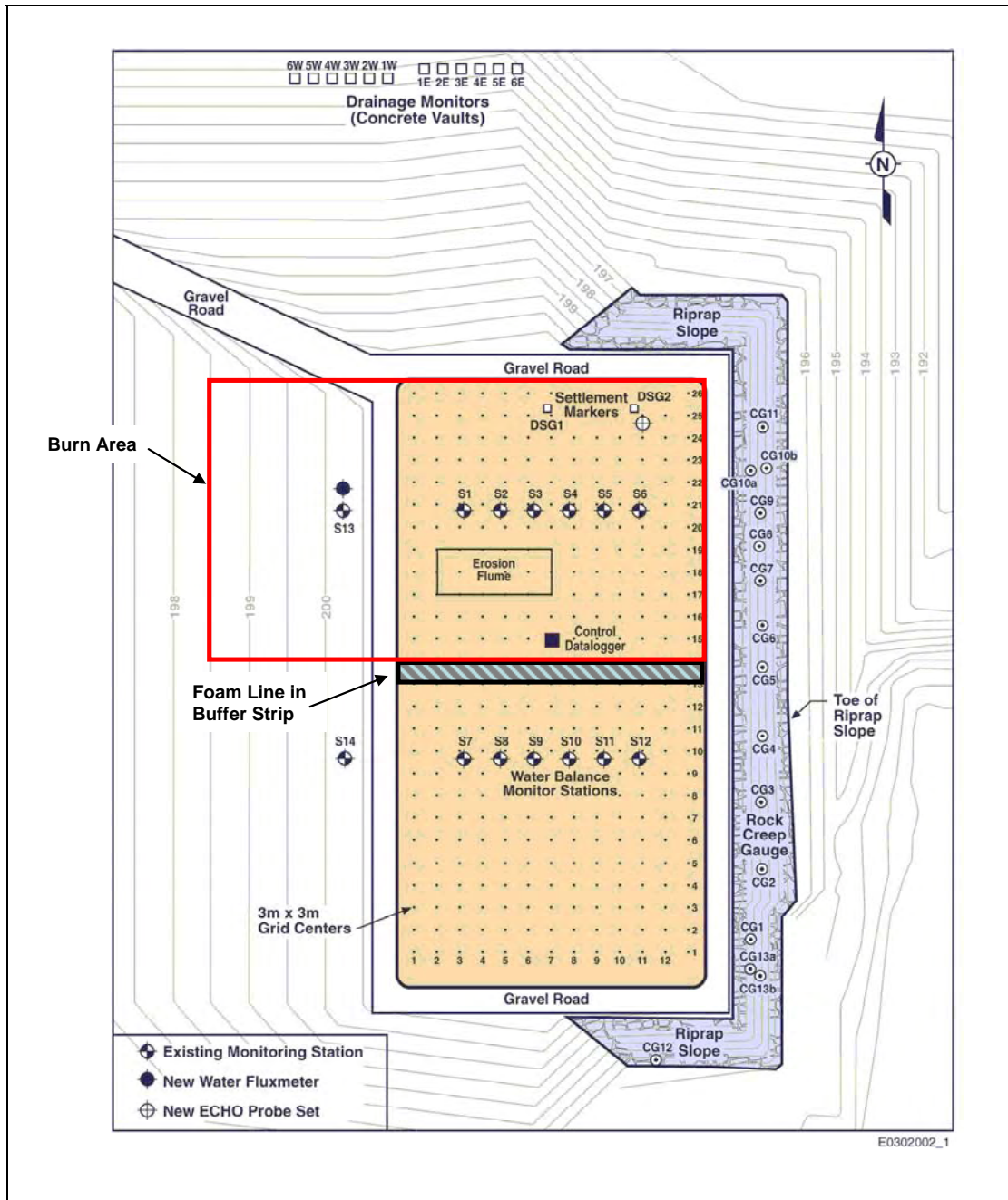
Figure 3.5. Schematic Plan View of the Barrier's Surface Showing Proposed Burn Area on the Gravel Side Slope and Silt-loam Surface. A 3 m wide line of fire retardant foam will be used to protect the south portion of the barrier during the burn.
